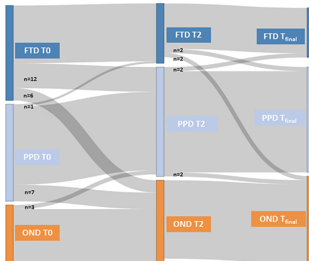
FIGURE 2. Patients that switched diagnosis between T0 and T2 and T2 and T final . T0: bvFTD n = 55, PPD n = 51, OND n = 31 and unknown n = 0. T2: bvFTD n = 29, PPD n = 54, OND n = 38 and unknown n = 16. T final : bvFTD n = 33, PPD n = 54, OND n = 46 and unknown n = 4. Abbreviations: FTD: frontotemporal dementia; PPD: primary psychiatric disorders; OND: other neurological disorders. T0 = baseline visit, T2 = follow-up visit 2 years after baseline, T final = 5–8 years after baseline visit.
