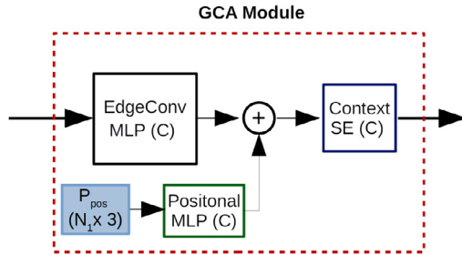
Fig. 5. The architecture of the proposed GCA module.
