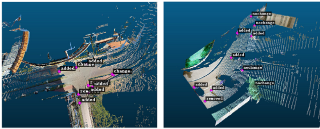
Fig. 1. Examples of the dataset showing city scenes with a variety of changed urban objects: left point cloud captured by LiDAR and the right point cloud generated by the simulator.
