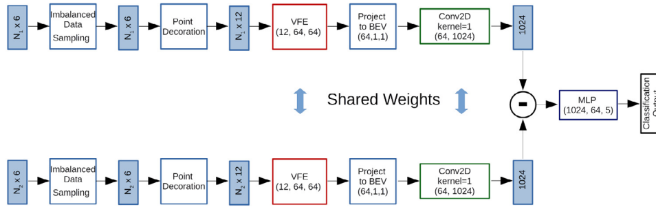
Fig. 7. The network architecture of the proposed SiamVFE method.
