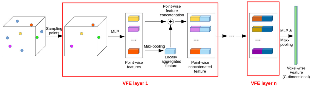
Fig. 6. Block diagram of the Voxel Feature Encoding (VFE).
