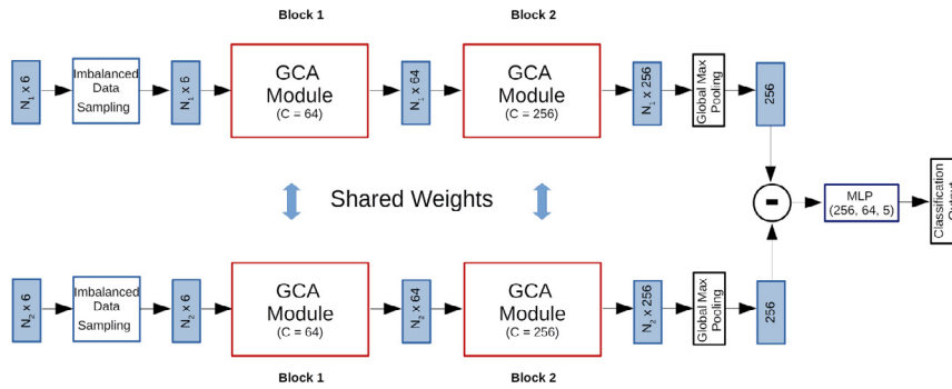
Fig. 4. The network architecture of the proposed SiamGCN-GCA method.
