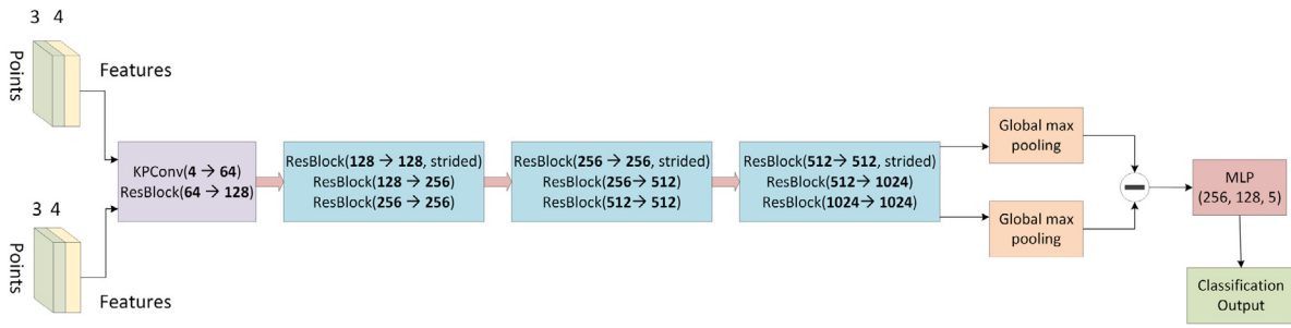
Fig. 8. The network architecture of the proposed SiamKPConv.
