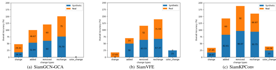
Fig. 9. The performance of different methods in terms of OA.
