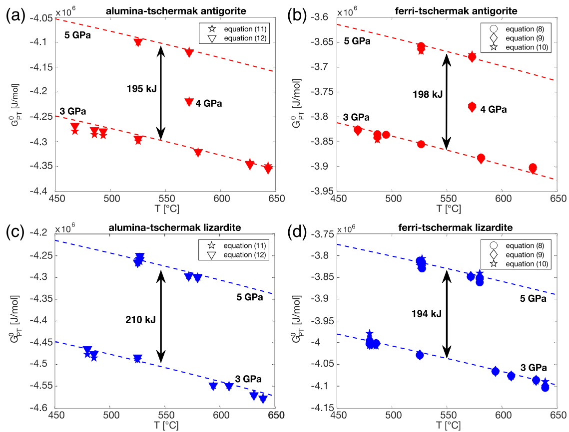
Fig. 7. The Gibbs energy of the new Al- and Fe 3+ -endmembers for antigorite (a, b) and lizardite (c, d). The symbols mark experimentally determined free energies obtained by fitting Eqs. (8)–(12) to the experimental results. The lines show the free energy obtained from linear combinations given in Table 3.
