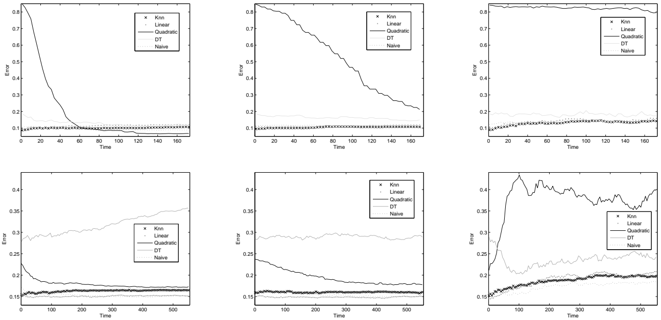
Figure 3: Error progression with sequential processing of new unlabelled data through the three online learning strategies: 'All' (left), 'Every n = 5 objects' (middle), and 'Window of fixed size' (right). From top to bottom, the figures correspond to thyroid and australian data sets.
