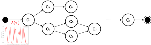
Figure 1. Application DAG.
