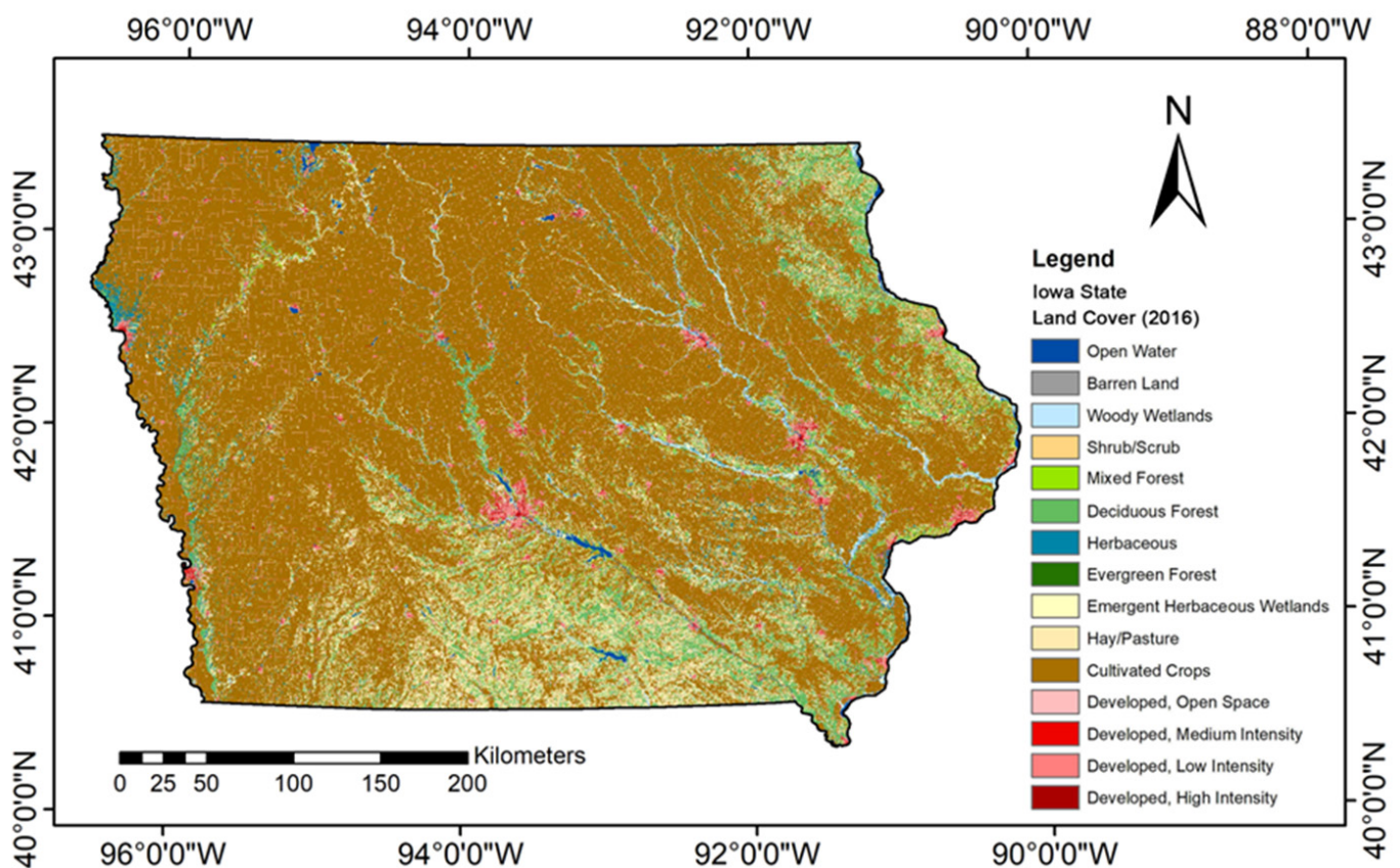
Figure 5. State of Iowa (IA) (USA) 2016 land cover map (40° 36' N to 43° 30' N and 89° 5' W to 96° 31' W) (using data from MRLC [31]) showing dynamic soil quality (soil health).
