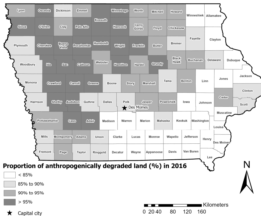
Figure 6. Anthropogenically degraded land proportion (%) by county in the state of Iowa (IA) (USA) in 2016. The proportion of land subject to anthropogenic degradation was calculated as a sum of developed land (developed, open space; developed, high intensity; developed, medium intensity; developed, low intensity), agriculture (cultivated crops, and hay/pasture), and barren land.
