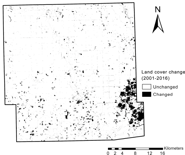
Figure 11. Dallas County, Iowa (IA), USA. Areas that changed land cover between 2001 and 2016 indicate potential damage to soil quality, notably in the area adjacent to the city of Des Moines.
