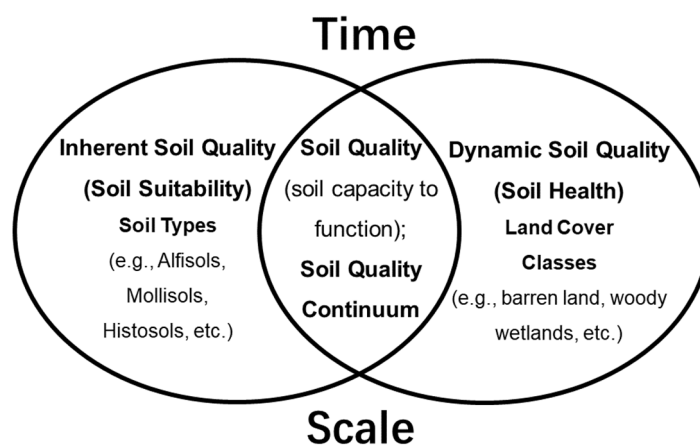
Figure 3. Soil quality is concisely defined as the soil’s capacity to function [5], which can be understood as the intersection of land cover and/or land use/land cover (LULC) change and soil type and over scale and time (adapted from Karlen et al., 2019 [25]). The SQ continuum is a series of values that differ with LULC and soil type.
