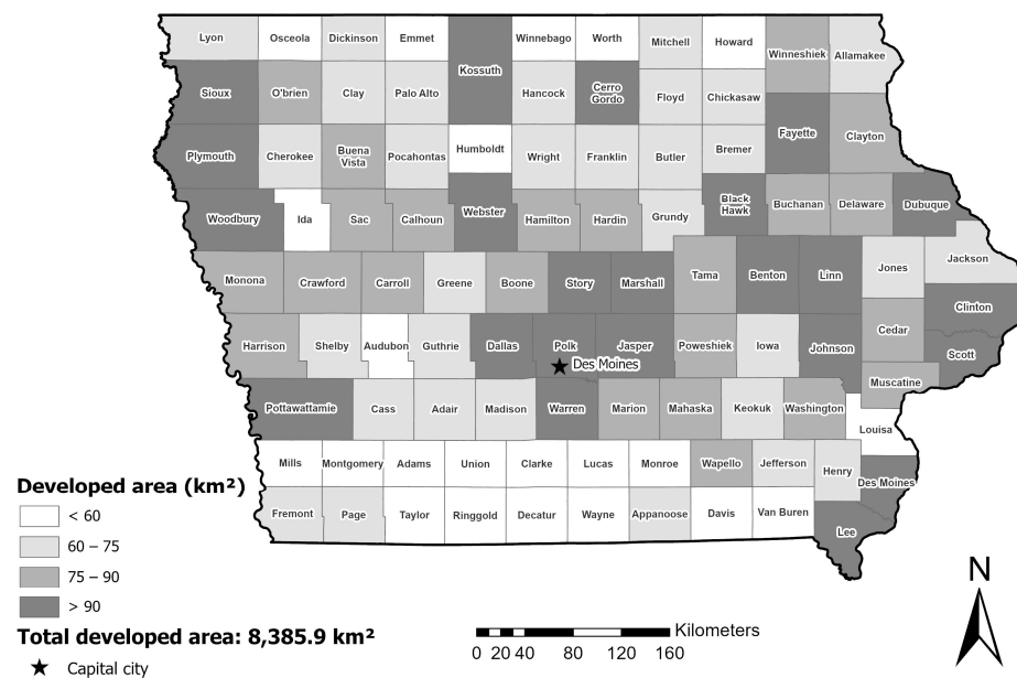
Figure 9. Damages to soil quality (SQ) from the loss of land for potential soil carbon (C) sequestration from past developments (through 2016) in Iowa (IA) (USA).
