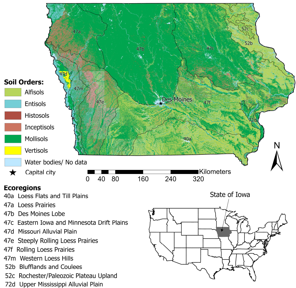
Figure 2. Soil map for the state of Iowa (IA), USA, ( 40^{\circ} 36' N to 43^{\circ} 30' N and 89^{\circ} 5' W to 96^{\circ} 31' W ) developed using the SSURGO spatial soils database [14] and ecoregions [15]. It shows the spatial distribution of soil orders with different inherent soil qualities (soil suitability). The inherent soil quality of IA is dominated by soil orders of Mollisols (60.9%) and Alfisols (23.9%), which are often inherently high-fertility soils important for agriculture.
