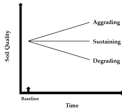
Figure 4. Concept of soil quality trends with time (adapted from Seybold et al., 1998 [26]).
