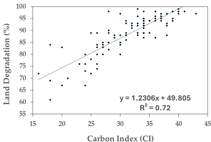
Figure 7. Relationship between the average carbon index (CI) of mineral soils for each county in Iowa [36] and the proportion of land degradation (%) in that county (determined in this study).
