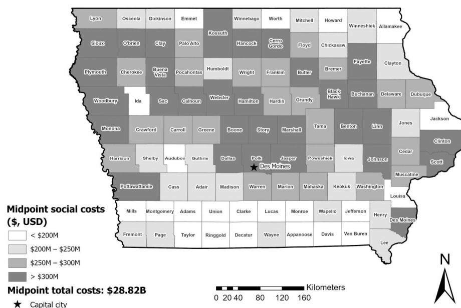
Figure 10. Damage to soil quality (SQ) from emissions can be measured as “realized” social costs of soil carbon (C) (SC-CO 2 ) from past developments (prior and through 2016) in the state of Iowa (IA) (USA). Note: M = million = 10 6 ; B = billion = 10 9 .
