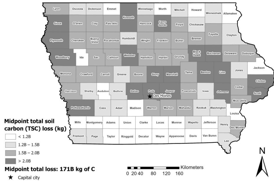
Figure 8. Soil quality (SQ) damage from soil carbon (C) loss with emissions associated with past land developments (through 2016) in Iowa (IA) (USA). Note: B = billion = 10^9 .
