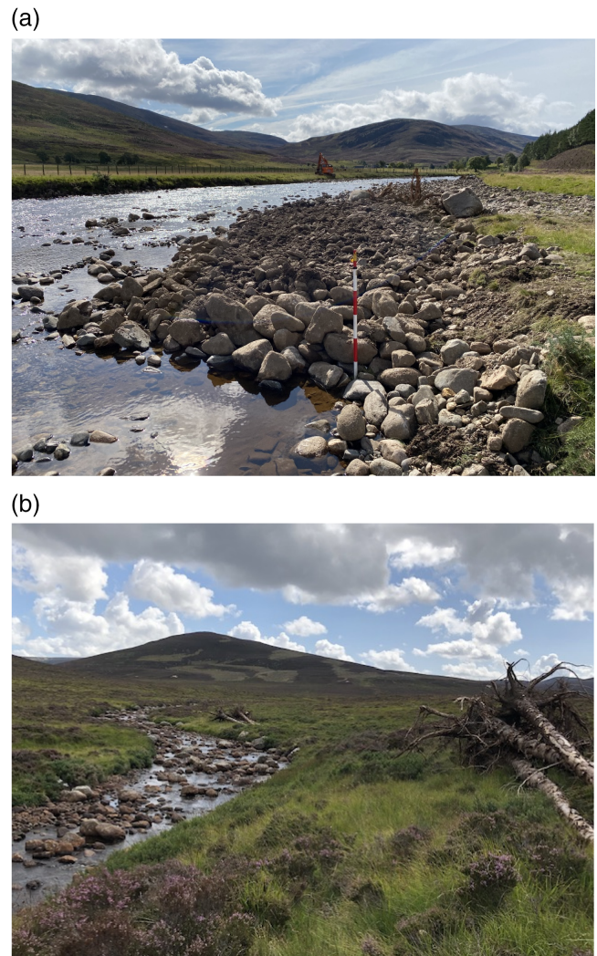
FIGURE 3 (a) A Large Wood Structure installed on a lateral bar in a salmon-bearing stream in the Cairngorms National Park. The exposed root bole is to the centre-right of the image just to the left of the large boulder in the river bank. The excavated area from the heavy plant (visible upstream) is in the foreground. (b) Trees located adjacent to stream prior to installation in area of juvenile salmon habitat.
