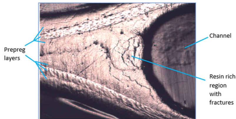
Figure 5. Microscope image showing fracture of microvascular channel following testing, modified from Dias et al. 2022 [15]
