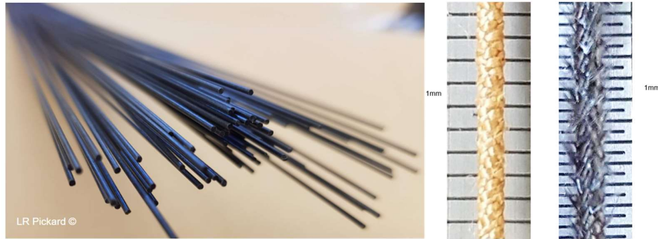
Figure 4. Micro overbraiding of pultruded rods. Left: carbon-fibre epoxy rods of 0.8 mm diameter. Centre: rod with 273 dtex PBO overbraid. Right: Rod with 1k T300 fuzzy carbon overbraid [4].
