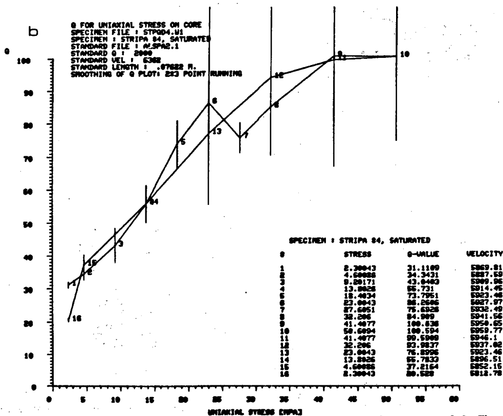
Fig. 7.20 a) Q_\alpha for specimen #4 from borehole DBEX-1 at the isotherm of 130° C. The specimen is dry and the Q_\alpha is a function of the uniaxial stress. Table of the test number, stress, Q-value and the V_p . b) Q_\alpha for specimen #4 from borehole DBEX-1 at the isotherm 130° C. The specimen is saturated and the Q_\alpha is a function of the uniaxial stress. Table of the test number, stress, Q-value and the V_p .
