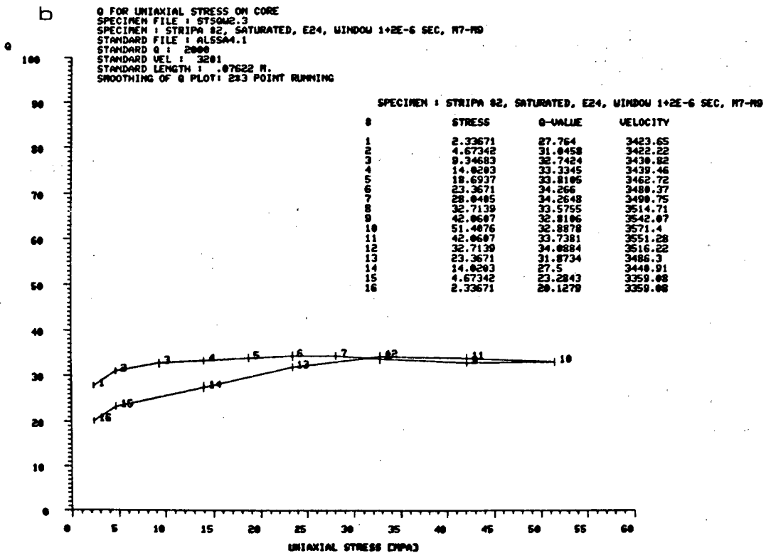
Fig. 7.23 b) Q_p for specimen #2 in a dry state. b) Q_p for specimen #2 in a saturated state.
