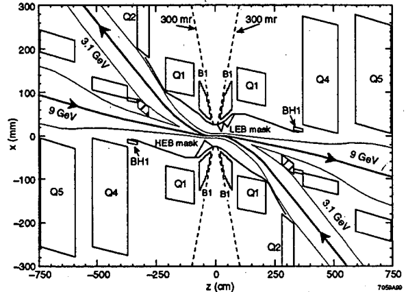
Fig. 2. PEP-II IR layout (anamorphic plan view).
