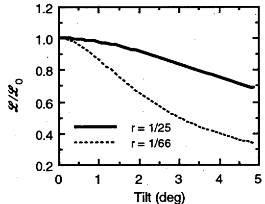
Fig. 3. Sensitivity of luminosity to relative beam tilt.
