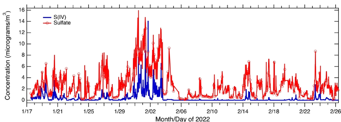
Figure 7. PILS-IC measurements of PM 2.5 sulfate and S(IV) measured at the CTC site. The IC separation resolves sulfate from S(IV) species (sulfite, bisulfite, and organo-sulfite adducts such as hydroxymethanesulfonate, HMS), which co-elute. HMS is a component of the S(IV) species. Note that the ratio of S(IV) to sulfate varies in time, being high in the cold event (late January/early February), but low in the warm event in late February.
