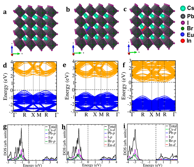
Figure 1. Schematic representation of the 3 \times 3 \times 3 supercell crystal structure of the (a) CsPbI 2 Br, (b) CsPb 0.96 Eu 0.04 I 2 Br, and (c) CsPb 0.96 In 0.04 I 2 Br and the corresponding (d–f) electronic band structures and (g–i) partial density of states.
