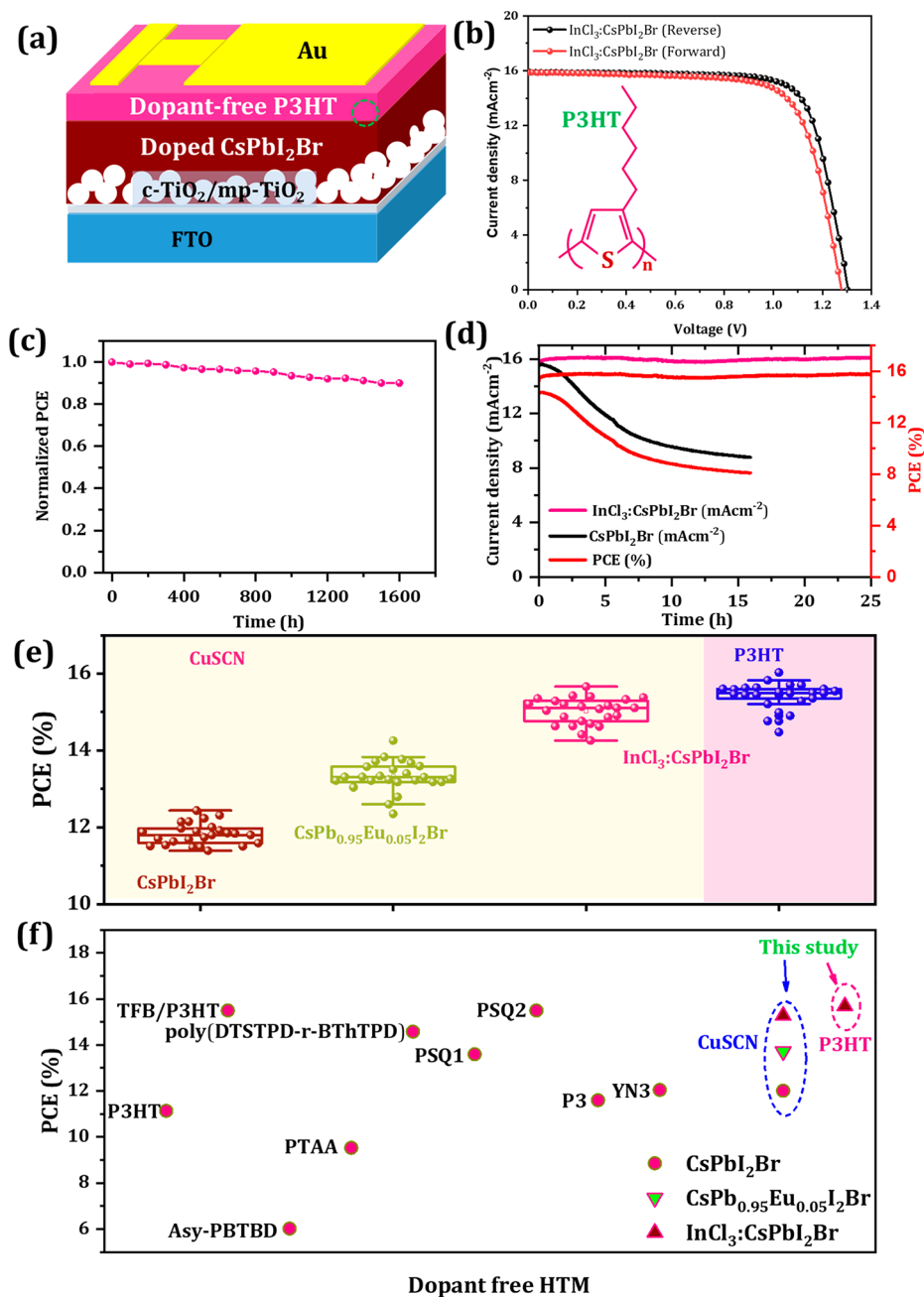
Figure 4. (a) Dopant-free P3HT HTL-based device configuration. (b) J - V characteristics of \text{InCl}_3 : \text{CsPbI}_2\text{Br} -based solar cells using dopant-free P3HT. (c) Ambient conditions device stability at 40–50% RH at 85 °C thermal stress of the 5 devices. (d) Steady-state current density and PCE of unencapsulated \text{CsPbI}_2\text{Br} and \text{InCl}_3 : \text{CsPbI}_2\text{Br} devices monitored under continuous 1.5 AM solar-simulator illumination as a function of time. (e) Device performance distribution for dopant-free HTLs for \text{InCl}_3 : \text{CsPbI}_2\text{Br} -based PSCs. (f) Distribution of PCE based on different dopant-free HTLs reported to date. Data has been extracted from refs 40, 43, 65, and 65.
