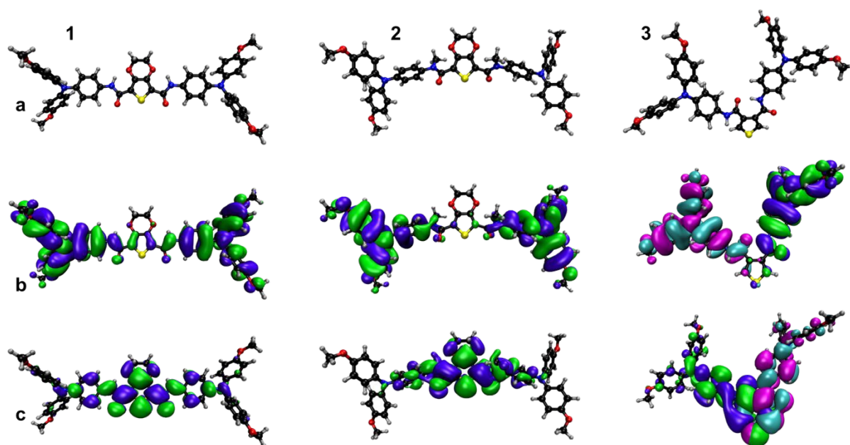
Figure 6: (a) Theoretical (PBE0/def2-sv(p)) optimised structures in DCM, overlaid with visualisations of (b) HOMO and (c) LUMO of our three amide HTMs. For 3 , we additionally show the destabilised HOMO-1 (-5.16 eV) and stabilised LUMO+1 (-1.18 eV) orbitals in cyan and magenta due to hydrogen bonding across the thiophene core.
