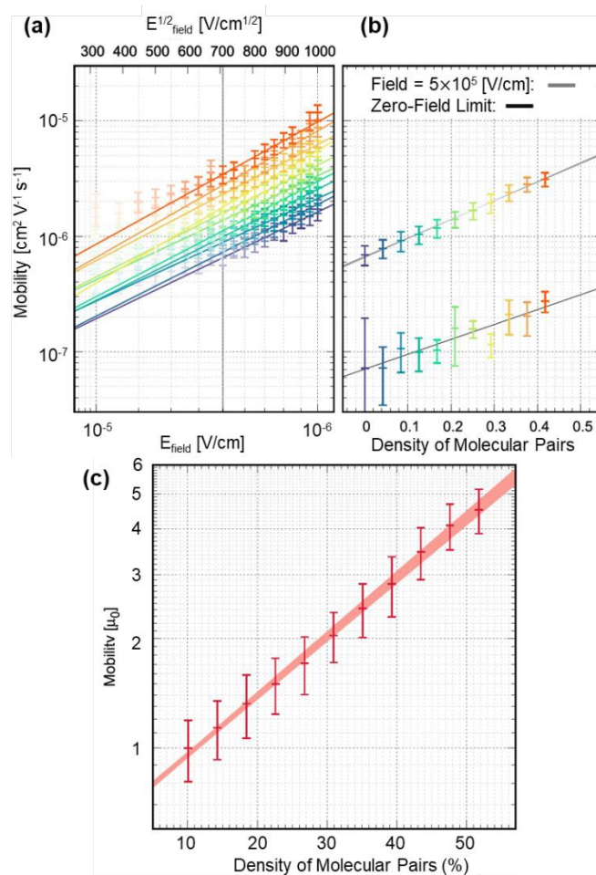
Figure 10: (a) Mobility against field at different pair densities, (b) mobility against pair density at a field strength of 5 \times 10^5 Vcm -1 and at zero field, (c) normalised mobility against pair density.
