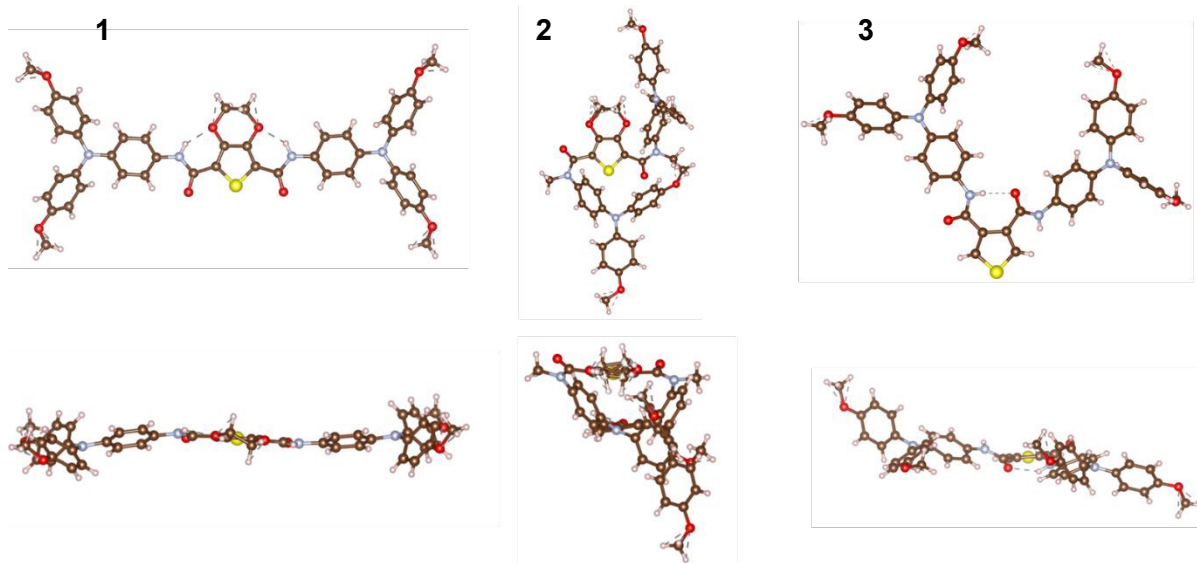
Figure 7: Top and side-on views of our three amide HTMs from the resolved X-ray crystal structure data. We note a vastly more twisted structure for compound 2 compared to that observed from DFT.
