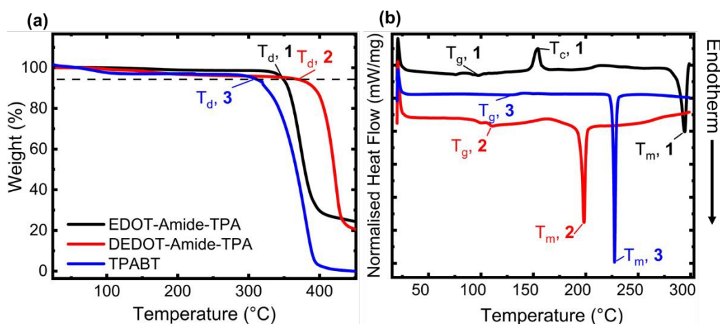
Figure 2: Stacked (a) TGA and (b) DSC curves for our three amide HTMs. Thermograms were recorded for pristine HTMs, at a rate of 5°C/minute under nitrogen.
