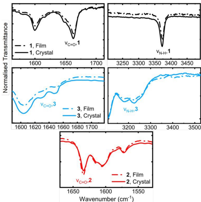
Figure 9: Comparative FTIR spectra of our three amides measured from either spin coated films (dotted lines) or from crystals (solid lines).
