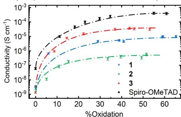
Figure 12: Estimated conductivities of our HTMs with increasing extent of oxidation. Dashed lines added only to guide the eye.
