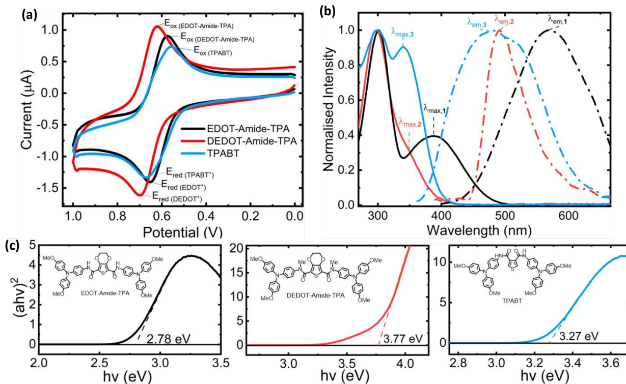
Figure 1: (a) Cyclic voltammograms referenced to the Fc/Fc^+ redox couple ( CH_2Cl_2 , 1 \times 10^{-4} M), (b) solution UV-Visible absorption (solid lines) and emission spectra (dashed lines) of the three amide-based HTMs, and (c) Tauc plots and corresponding optical bandgaps E_g .
