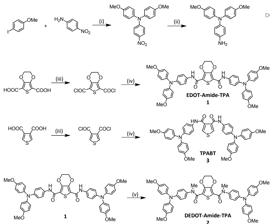
Scheme 1: Condensation chemistry-based syntheses of the three HTMs used in this study. (i): K_2CO_3 , copper powder, 18-crown-6, DMF, reflux (150 °C, 16 hours), yield 67%; (ii): 10% palladium on carbon, hydrazine hydrate, dry THF, reflux (66 °C, 16 hours); (iii): thionyl chloride, THF, reflux (66 °C, 2 hours); (iv): 4-amino-4',4''-dimethoxytriphenylamine, triethylamine, THF, room temperature, stir overnight, yield 70%; (v): sodium hydride, dry THF, iodomethane, 40 °C, overnight, yield 48%.
