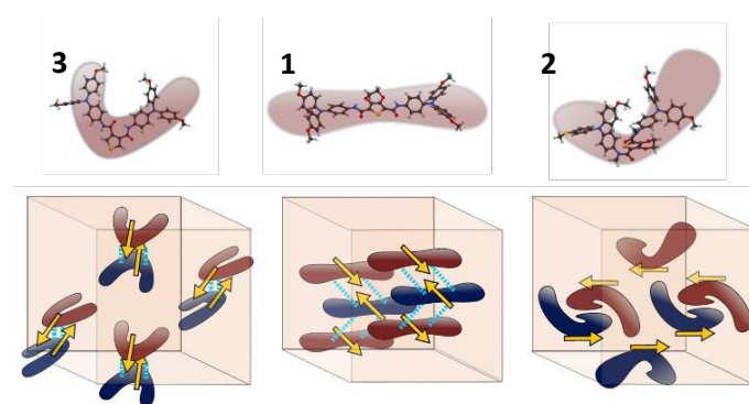
Figure 8: Graphical representation of the crystal structure packing of compounds 1-3 .
