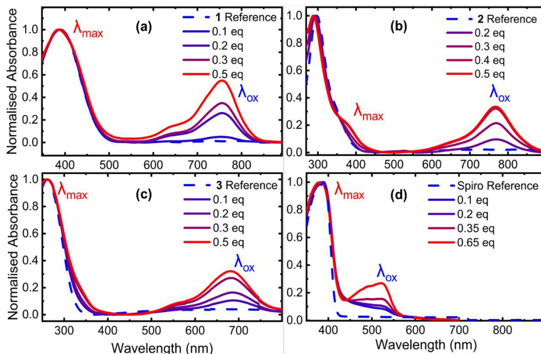
Figure 11: Doping trends in the film UV-Visible absorption spectra of our amide-based HTMs (a-c) and spiro-OMeTAD (d), with increasing concentrations of FK209.
