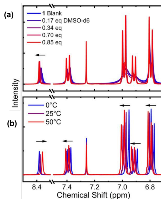
Figure 4: Partial NMR spectra showing the aromatic and amide proton region in compound 1 , (a) with increasing concentration of DMSO-d 6 , (b) with increasing temperature.
