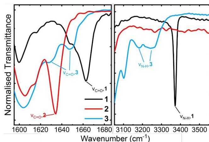
Figure 5: Partial FT-IR spectra obtained from powder samples of our three amides, showing the carbonyl stretch region (left) and the N-H stretching region (right).
