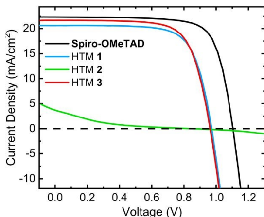
Figure 13: JV-Curves of our champion devices for each tested HTM, collected under AM 1.5 simulated sunlight.
