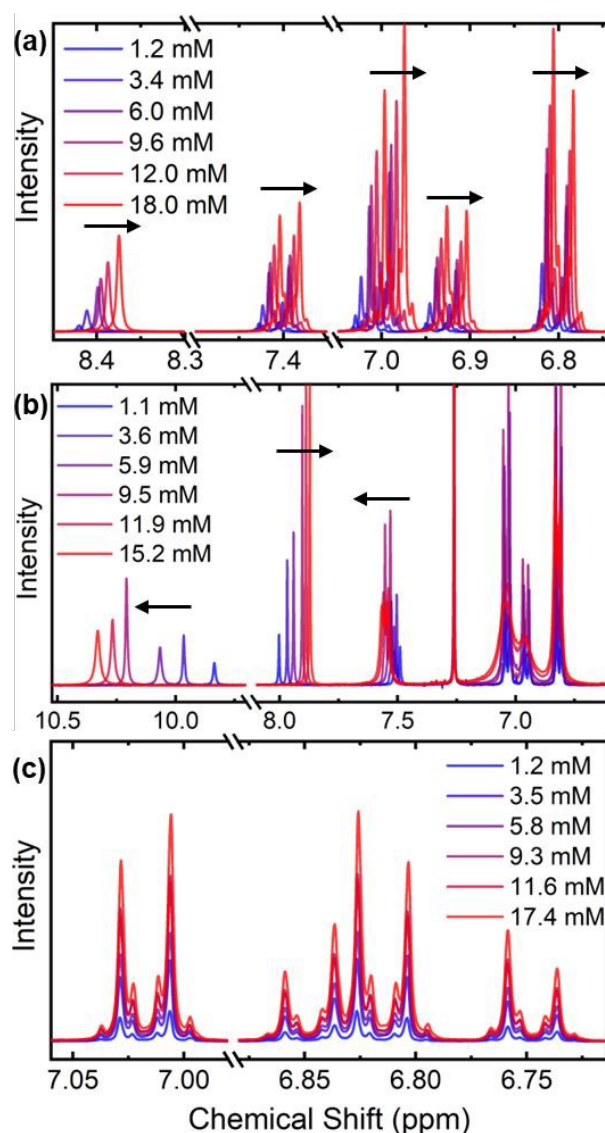
Figure 3: Partial 1 H-NMR spectra of (a) compound 1 and (b) compound 3 at different concentrations, showing shifts in their amide and aromatic proton resonances, and (c) compound 2, showing no shifts across the concentration range.
