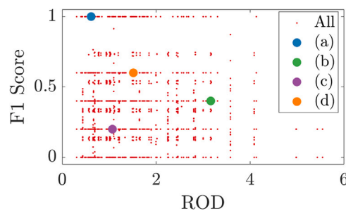
Fig. 12. Rank of domain (ROD) against F1 score on the target testing dataset. ‘All’ denotes feature set combinations that are not MCSs and (a), (b), (c) and (d) denote the MCS set.
