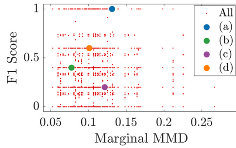
Fig. 13. Marginal maximum mean discrepancy (MMD) against F1 score on the target testing dataset. ‘All’ denotes feature set combinations that are not MCSs and (a), (b), (c) and (d) denote the MCS set.
