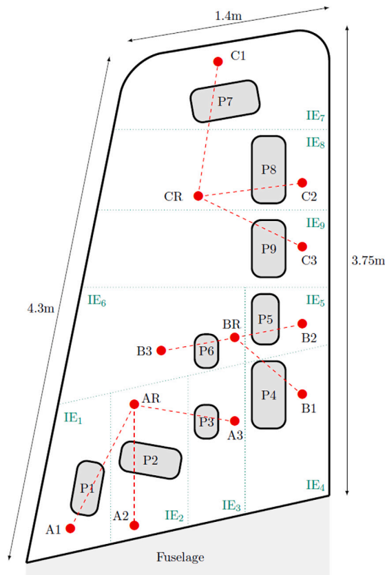
Fig. 1. Schematic of the Gnat aircraft wing and associated irreducible element model (not to scale).
