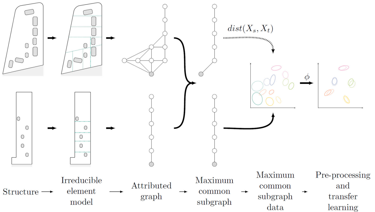
Fig. 5. Schematic overview of the population-based methodology.
