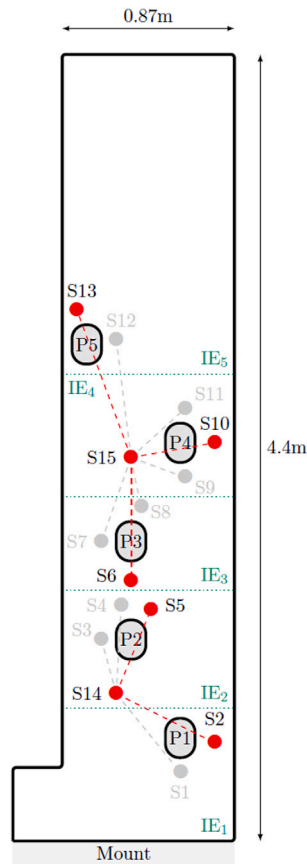
Fig. 2. Schematic of the Piper Tomahawk aircraft wing and associated irreducible element model (not to scale).
