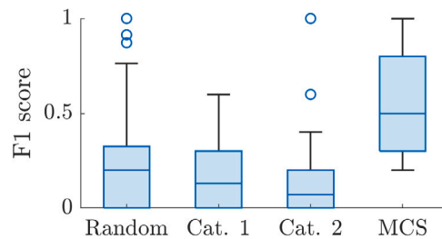
Fig. 11. Box and whisker plots of testing F1 scores from kNN classifiers trained on BDA latent spaces. ‘Random’ denotes feature set combinations that are not valid paths in the AGs, ‘Cat. 1’ are combinations that are valid paths in the AGs and ‘Cat. 2’ combinations that are valid paths and include the boundary condition nodes in the AGs.
