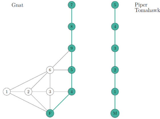
Fig. 6. Maximum common subgraph (a).
