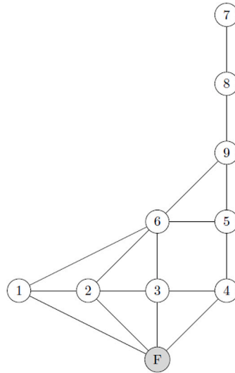
Fig. 3. Attributed graph for the Gnat aircraft wing. White and grey circles denote structural and boundary nodes respectively.
