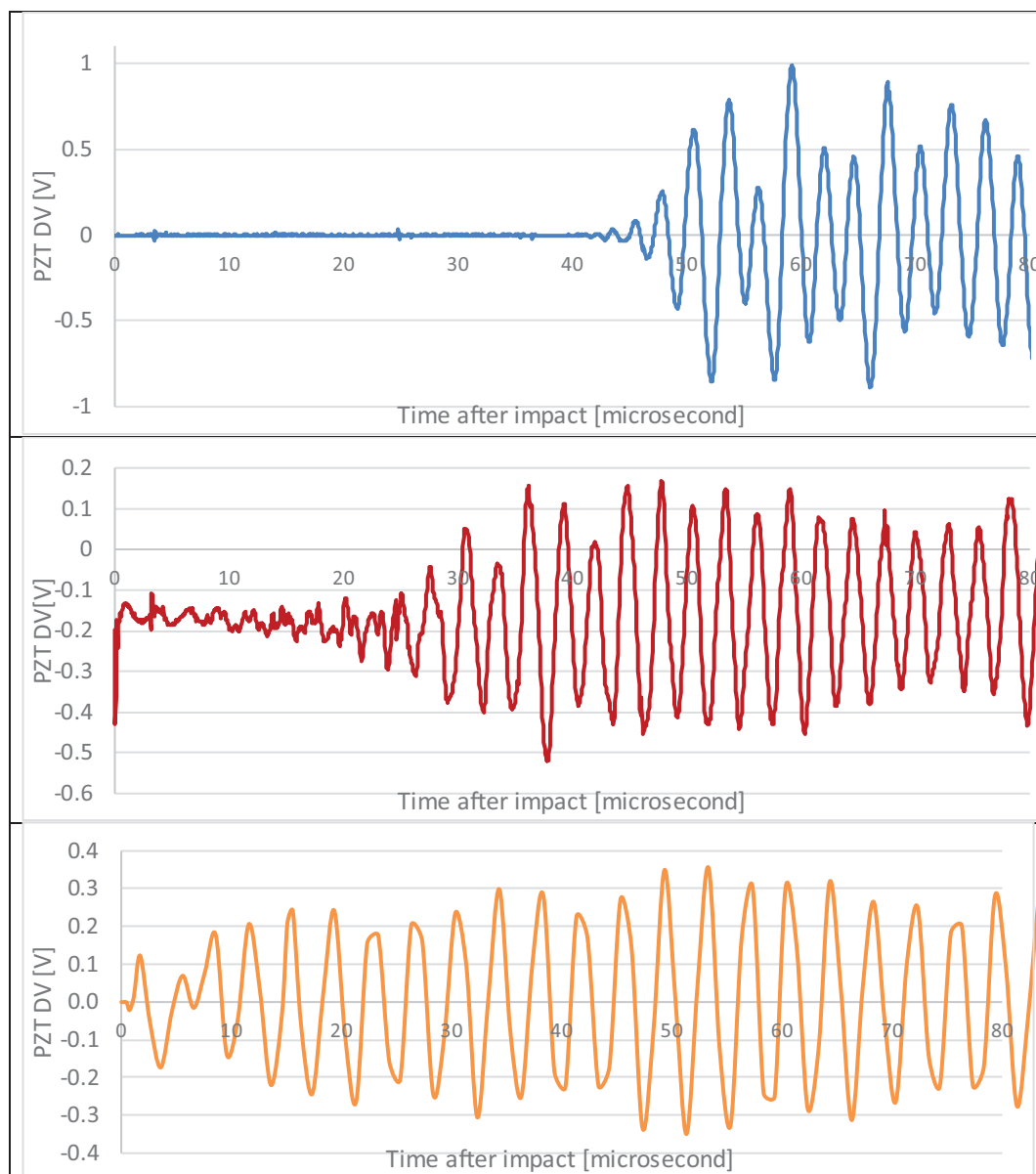
Fig. 8. Comparison between Lamb waves generated by: a 1 mm sphere impacting on the DISC breadboard sensing plate at about 0.01 km/s (upper panel); a laser simulated HVI on the DISC breadboard sensing plate (laser energy 50 mJ corresponding to a 50 \mu m particle at about 8 km/s) (middle panel); a numerical simulated HVI (25 \mu m particle at 15 km/s), on the DISC simulated sensing plate (lower panel). Signals start at different time because of the different distances from the PZT of the real or simulated impact.
