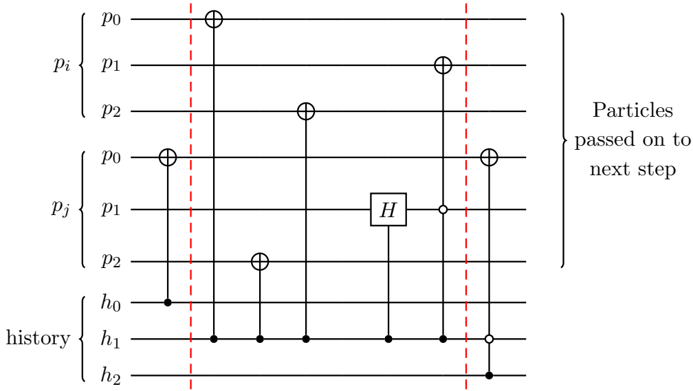
Figure 5.6: Update gate for the first step of the algorithm (taken from Reference [4]). Each slice is a different update mechanism: far left slice updates q \rightarrow qq splittings, centre slice updates g \rightarrow q\bar{q} and the far right slice updates g \rightarrow gg .
