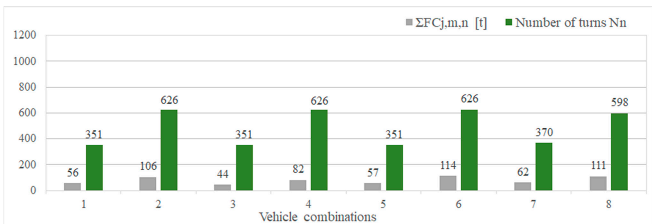
Figure 5. Estimated fuel consumption for considered vehicle combinations.
