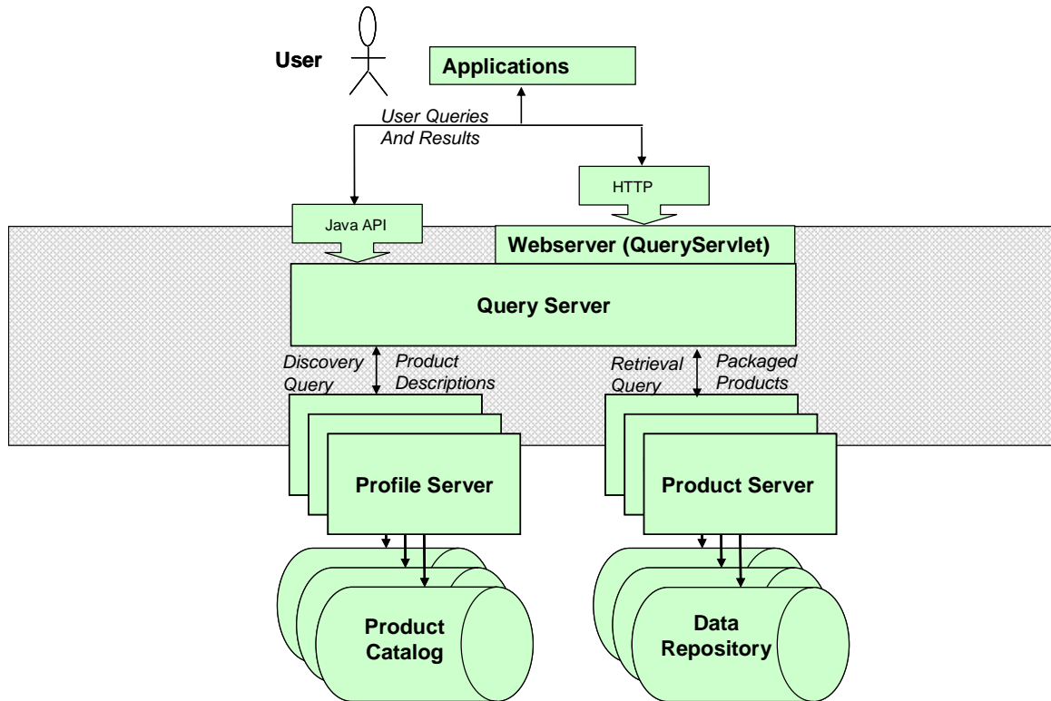
Figure 4. Software Framework Component Architecture
