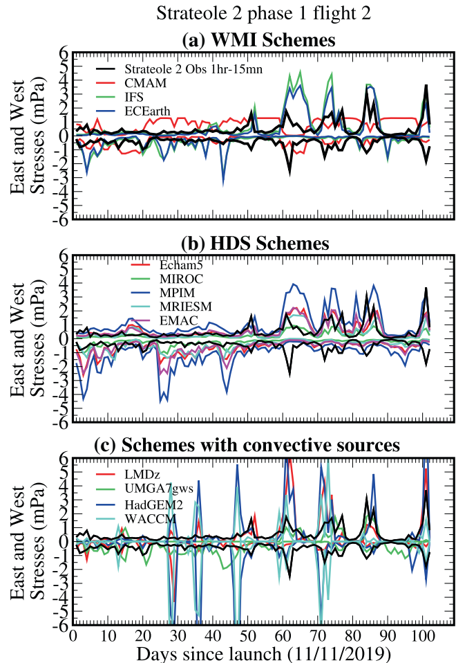
FIGURE 3 Comparison between daily averaged values of the eastward and westward MFs measured by balloons during Strateole 2 phase 1 Flight 2 and estimated by the GW schemes at the balloon location and altitude. Coloured curves are for the GW schemes using ERA5, black curves are for the observed MFs due to 15 min–1 h GWs. (a) WMI schemes; (b) HDS schemes; (c) schemes relating launched MFs to convective sources or precipitation: all multiwaves except UMGA7gws. [Colour figure can be viewed at wileyonlinelibrary.com ]
