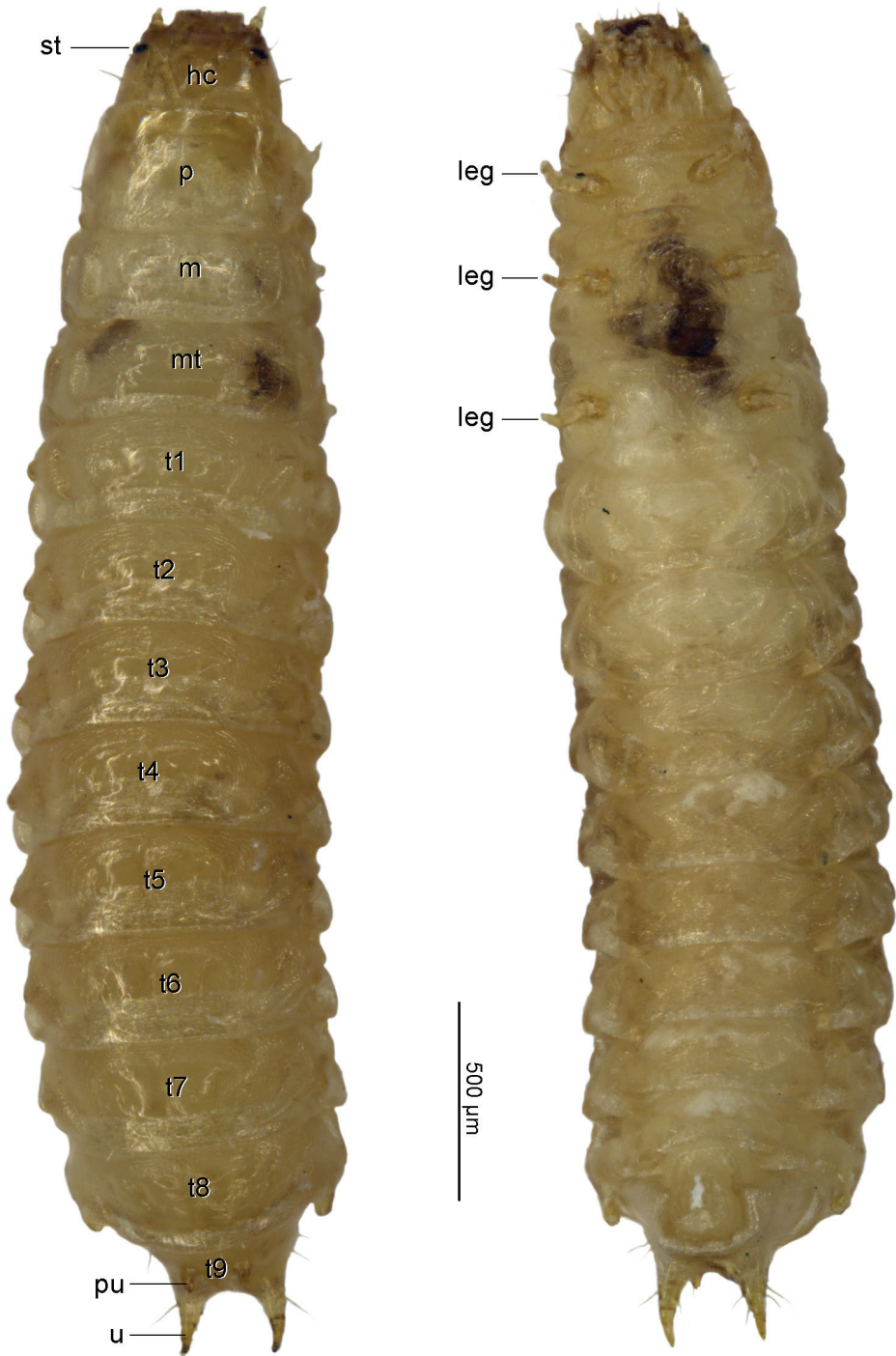
Figure 3. Omosita nearctica larva – dorsal (L) and ventral (R) views. hc = head capsule m = mesothorax, mt = metathorax, p = prothorax, pu = pregomphus, sp = spiracle, st = stemmata, u = urogomphus, 1–9 = abdominal tergites. Scale bar: 0.5 mm.
