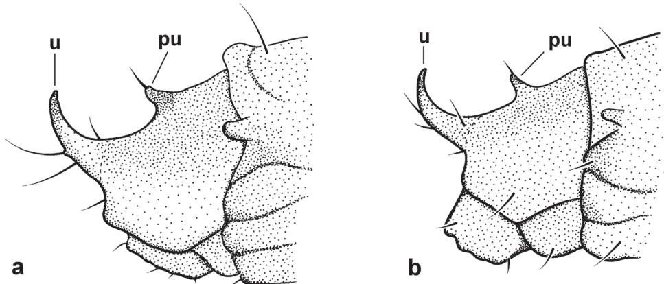
Figure 9. Lateral view of terminal end of Omosita nearctica ( a ) and O. colon ( b ). pu = pregomphus, u = urogomphus. Not to same scale.
