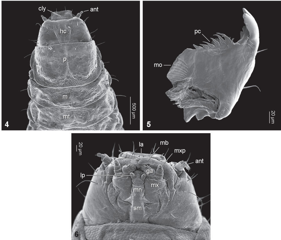
Figures 4–6. 4 SEM dorsal view of head capsule and thorax of Omosita nearctica larva. ant = antenna, cly = clypeus, hc = head capsule, m = mesothorax, mt = metathorax, p = prothorax 5 SEM ventral view of left mandible of Omosita nearctica larva. mo = mola, pc = prostheca 6 SEM ventral view of head of Omosita nearctica larva. ant = antenna, la = labrum, lp = labial palp, mb = mandible, mn = mentum, mx = maxilla, mxp = maxillary palp, sm = submentum. Scale bars: 500 µm ( 4 ), 20 µm ( 5 , 6 ).
