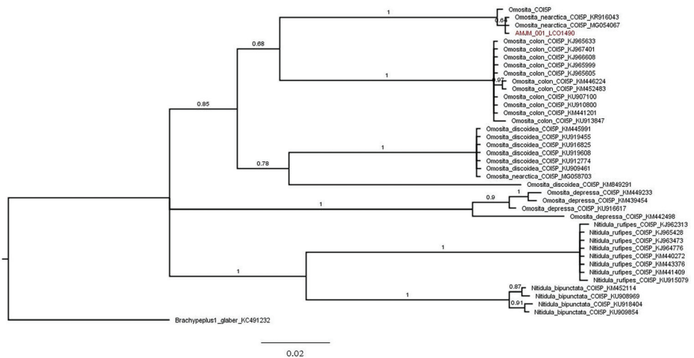
Figure 2. Bayesian inference tree of COI sequences. Posterior probability values are shown on branches. Red text is the South African sequence generated in this study.
