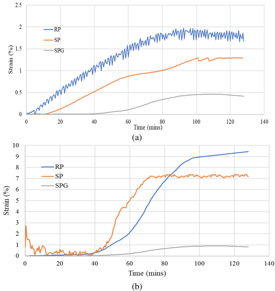
Figure 11: Representative strain development over time for RP, SP, and SPG for a) the gluelines, and b) the board.
