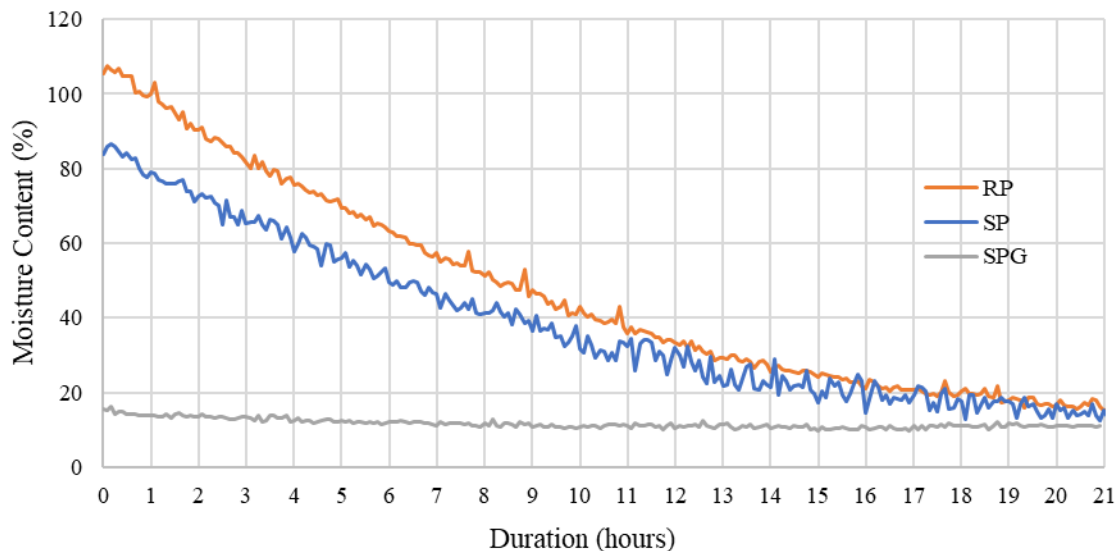
Figure 8: Average drying curves for MC change over time of RP, SP, and SPG samples.
