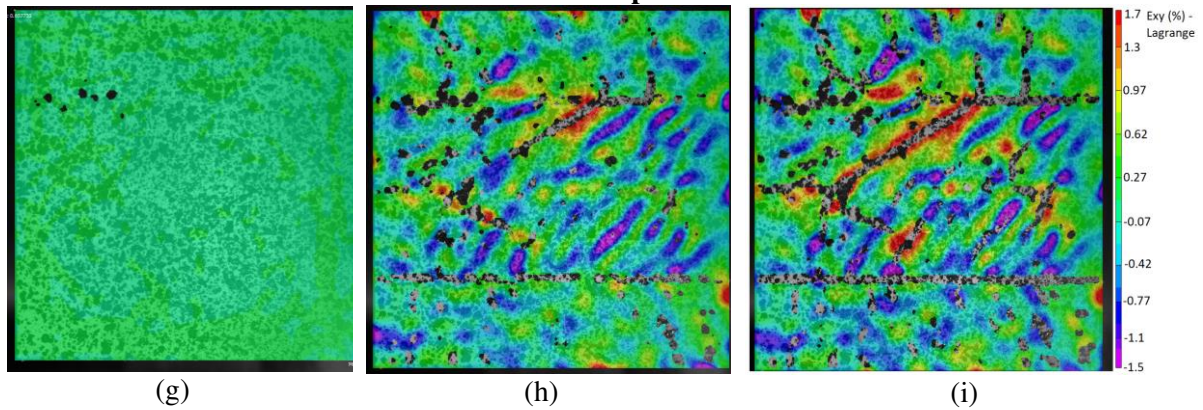
Figure 9: DIC output images from \epsilon_{xy} strain field for a RP sample at (a) 30 mins, (b) 8, (c) and 21 hours, a SP sample at (d) 30 mins, (e) 8, and (f) 21 hours, and a SPG sample at (g) 30 mins, (h) 8, (i) and 21 hours.
