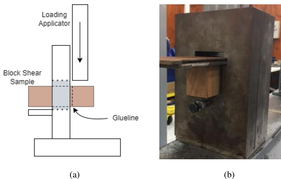
Figure 6: (a) Block shear schematic, and (b) testing setup.
