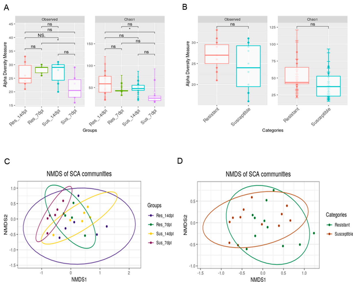
Figure 2. Alpha diversity of the gut microbiome communities in sugarcane aphids (SCA) subjected to different days of infestation on resistant and susceptible sorghum plant lines without endosymbiont bacteria, Buchnera aphidicola . Diversity was assessed using observed operational taxonomic units (ASVs), and Chao1. Boxplots of bacteria richness and diversity indices within infestation groups (A) and by plant categories (B). Non-metric multidimensional scaling (NMDS) plots showed variations in microbiome composition among groups (C) and no statistical difference among categories (D). The colours used in Figure 2 are not meant to represent the same thing. After removing the primary endosymbiont bacteria, B. aphidicola , all samples were rarefied to a sequence depth of 49 reads before being subjected to diversity analysis. p -value ( 0.01 < * < 0.05 ). Res: resistant; Sus: susceptible; ns: no significance; dpi: days post infestation.
