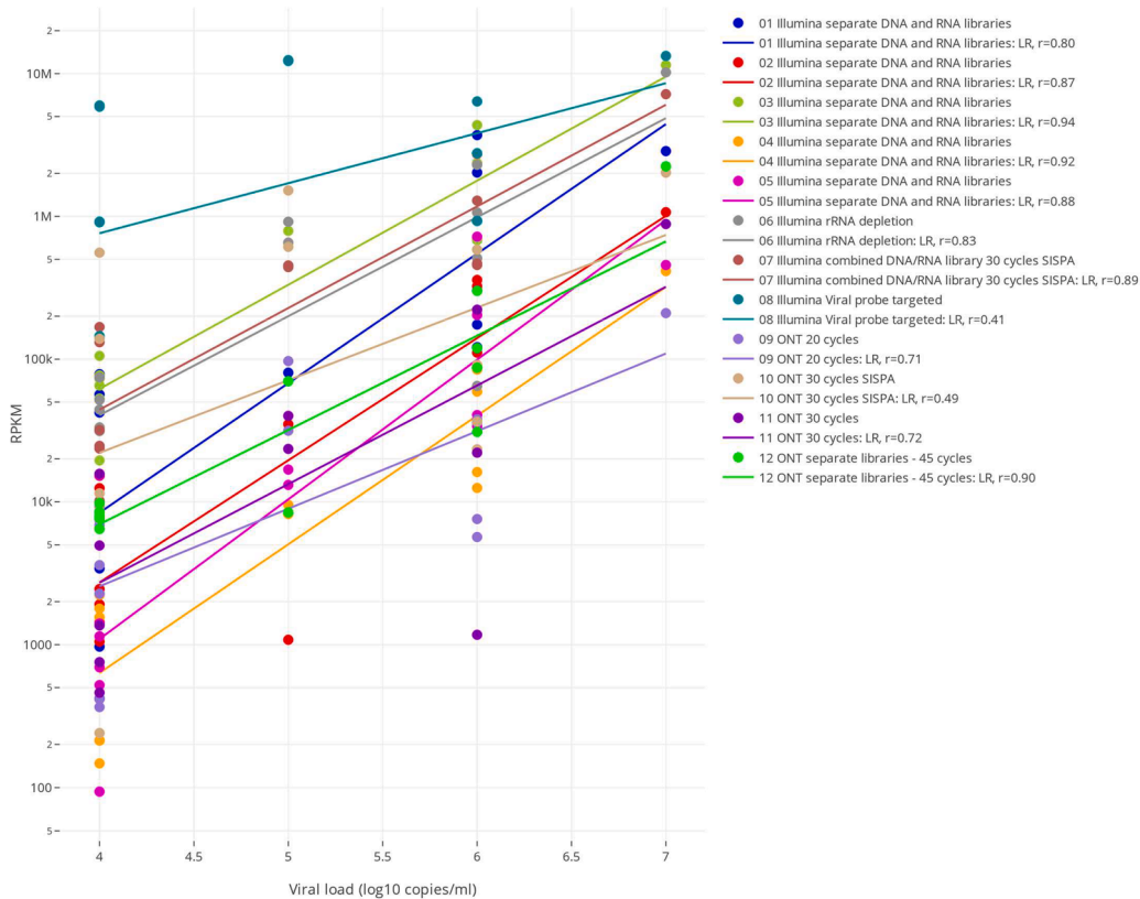
Fig. 2. Correlation between normalized sequence read counts (per kilobase per million, RPKM) and viral loads (copies/ml) for the protocols. Legend: LR; linear regression, r; Pearson's correlation coefficient, SISPA; sequence-independent single-primer amplification, ONT; Oxford Nanopore Technologies.
