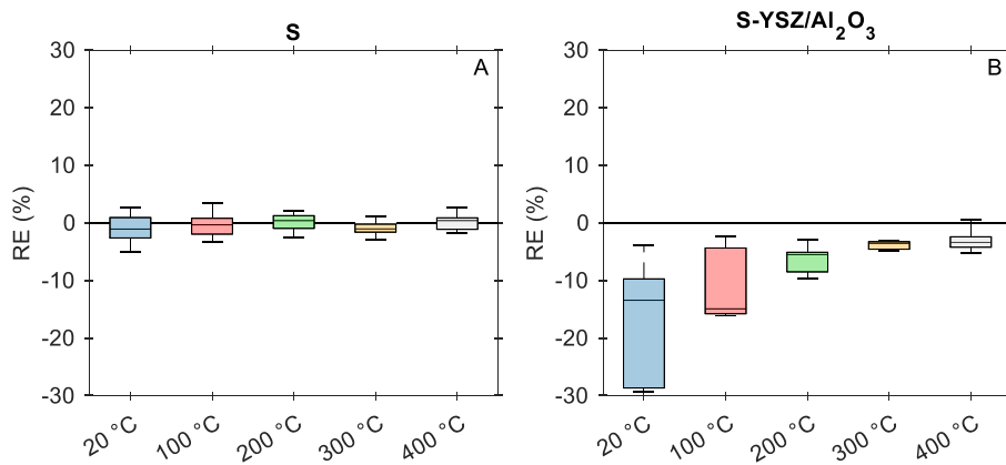
Fig. 9. Box plot showing the relative error of: A) the fitted and experimental data of the support (S) model and B) the experimental validation data and the model's predictions for the YSZ/Al 2 O 3 layer model. The experimental data was obtained in pure C 3 H 8 , CH 4 and CO 2 , at T = 20–400 °C and 1.5–4 bar(a).
