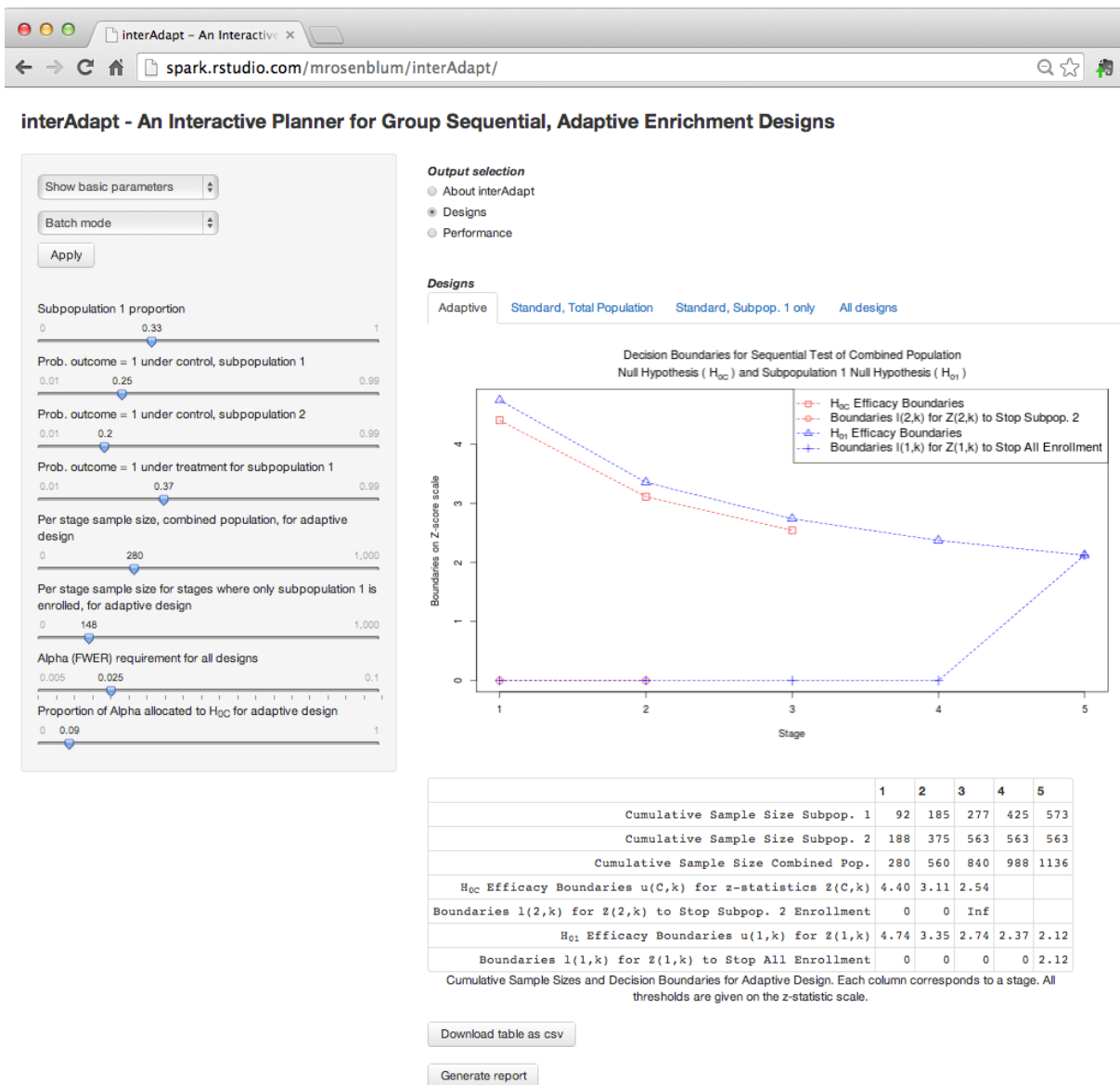
Figure 1: Designs Screenshot: Inputs can be entered in the side panel on the left, with results visible in the main panel on the right. The drop down menus at the top of the side panel can be used to navigate different interfaces to input parameters. Here we show the “Basic parameter” inputs, in “Batch mode,” where the Apply button must be pressed to update the results in the main panel. The radio buttons at the top of the main panel can be used to navigate between design outputs describing the decision rules for each trial, and performance summaries for each trial. In this figure we show the design for the adaptive trial ( AD ), based on the default input parameters. Boundaries for the z-statistics Z_{1,k} , Z_{2,k} and Z_{C,k} are shown both in the plot, and in the table. The table also contains information on how many participants are enrolled in each stage. The scroll bar on the right of the web browser has been cropped out of this figure for the sake of increased screenshot resolution.
