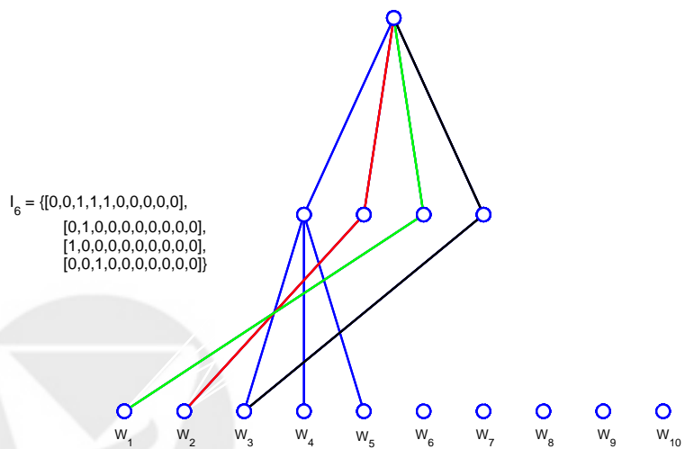
D/S/A Sequence for Friedman 1 Data: 6 Edges
