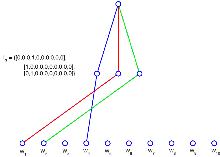
Figure 16: Friedman 1 simulation : D/S/A sequence-model with 3 lower edges.
