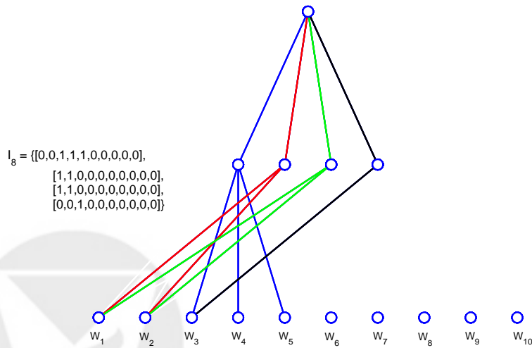
D/S/A Sequence for Friedman 1 Data: 8 Edges
