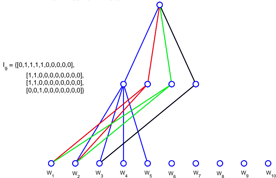
Figure 5: Friedman 1 simulation : Neural-network model selected by 5-fold cross-validated D/S/A algorithm.
