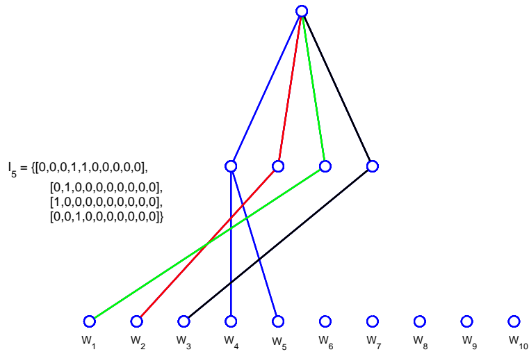
D/S/A Sequence for Friedman 1 Data: 5 Edges
