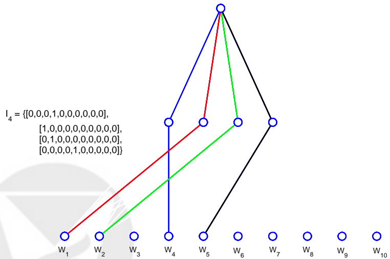
Figure 17: Friedman 1 simulation : D/S/A sequence-model with 4 lower edges.
