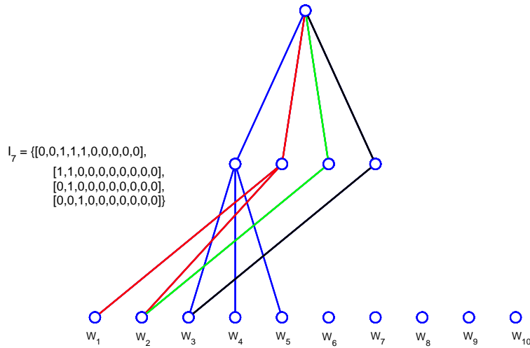
D/S/A Sequence for Friedman 1 Data: 7 Edges
