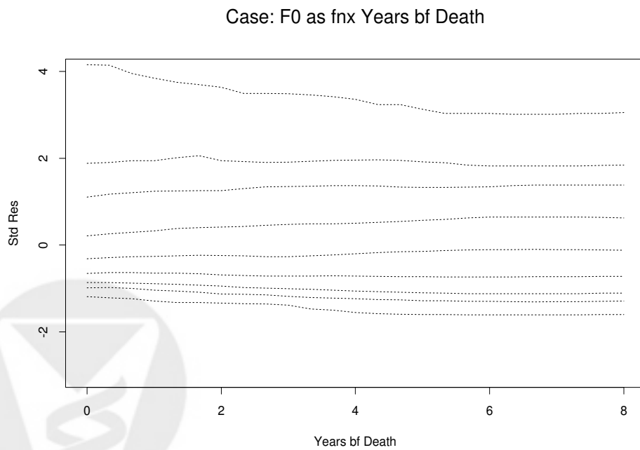
Figure 4: (a) Estimated quantiles of F_0 based on the kernel estimation method. F_0 is allowed to depend on age.(b) Estimated quantiles of F_0 based on the kernel estimation method. F_0 is allowed to depend on years before death.
