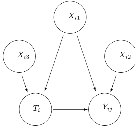
Figure 1: Casual diagram for simulation study
