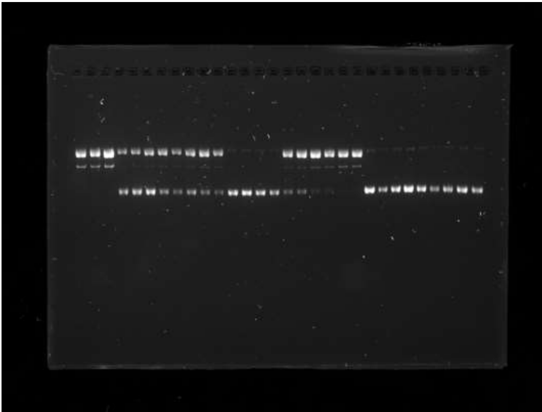
Supplementary Figure 1. Full, uncropped gel electrophoresis image from which Figure 3 was cropped. Figure 3 includes bands 4 – 14 as a representation of how increased dose changes plasmid structure proportion.
