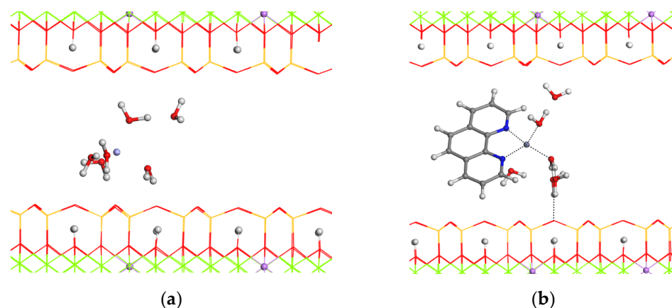
Figure 7. Zinc hectorite (a) and zinc hectorite with a phenanthroline molecule adsorbed in the interlayer space. (b) Oxygen atoms are depicted in red, hydrogen in white, silicon in yellow, magnesium in green, lithium in pink, zinc in light blue, nitrogen in blue, and carbon in gray. The H and Li atoms, and the interlayer atoms, are highlighted as balls.
