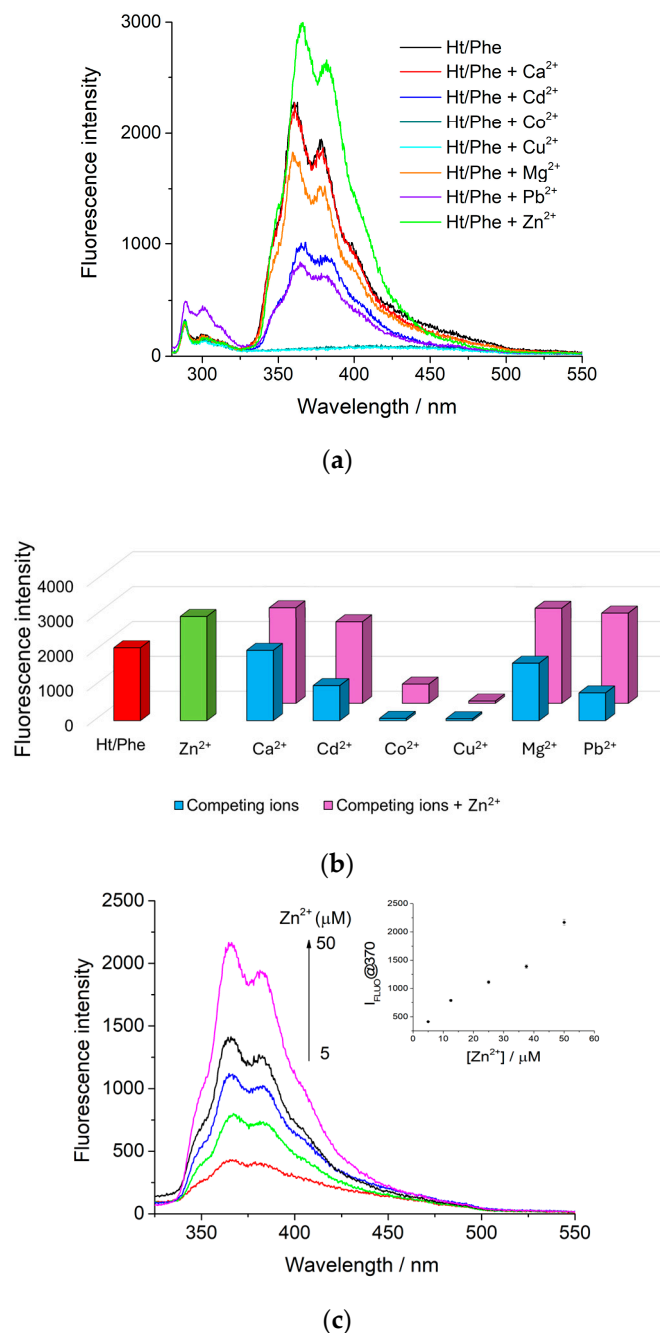
Figure 4. (a) Changes in fluorescence emission spectra ( \lambda_{\text{ex}} = 260 \text{ nm} ) of Ht/Phe ( 0.05 \text{ mg mL}^{-1} ) with addition of different metal ions ( 37.5 \text{ }\mu\text{M} ) in water; (b) fluorescence intensity of Ht/Phe nanomaterial in the absence (red bar) and in the presence of different metal cations ( 37.5 \text{ }\mu\text{M} ) with (pink bars) and without (blue bars) the addition of Zn 2+ ions ( 37.5 \text{ }\mu\text{M} ) in water, in green bar is reported the Ht/Phe fluorescence response to Zn 2+ addition; (c) fluorescence spectra of Ht/Phe nanomaterial upon addition of different concentration of Zn 2+ ions (5–50 \mu\text{M} ).
