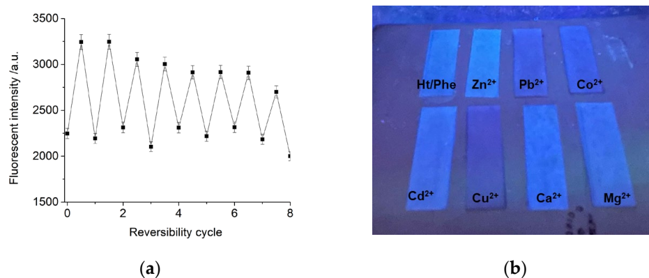
Figure 5. (a) Reversibility of Ht/Zn nanomaterial ( 0.05 \text{ mg mL}^{-1} ) upon sequentially adding \text{Zn}^{2+} and EDTA, \lambda_{\text{ex}} = 260 \text{ nm} (error bars represent SD ( n = 3 )); (b) photographs of test strips for detecting various cations under illumination at 265 \text{ nm} .
