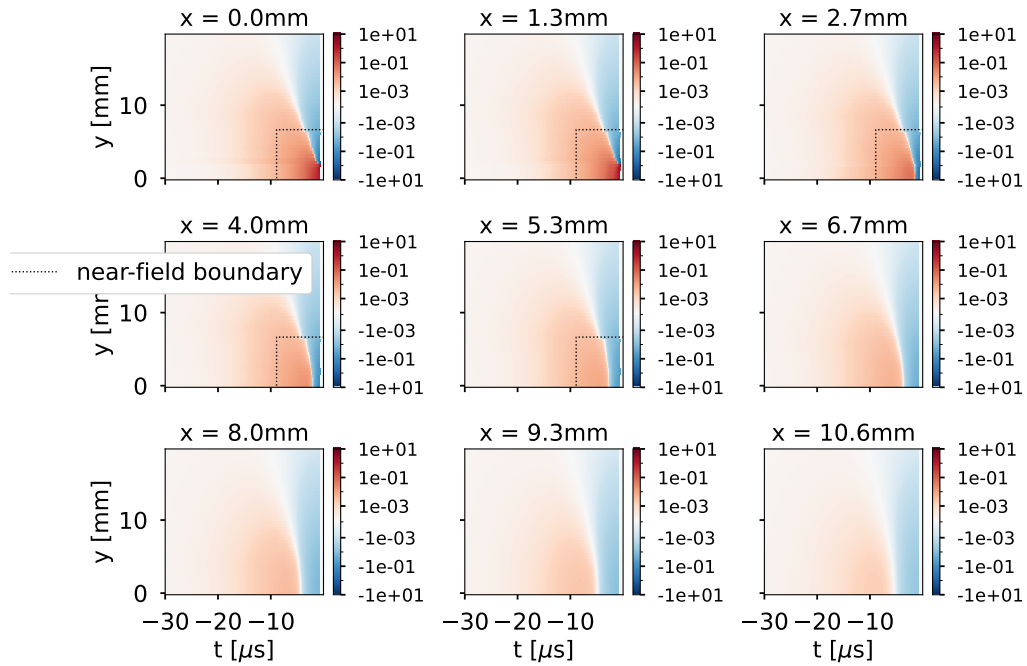
Figure 5. Induced current on a 4.4 mm pixel from a drifting electron at a given drift time and x, y position relative to the pixel, in units of electrons per 0.1 μs. The different calculations used for the near-field and far-field regions are described in the text in section 3.3.1 with the near-field boundary highlighted with a dotted line.
