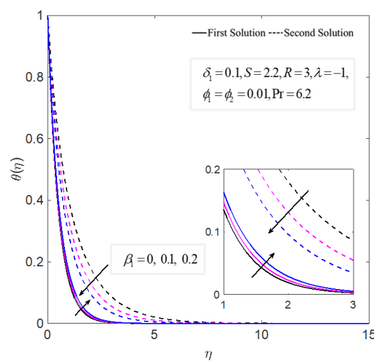
Fig. 9. Temperature profiles \theta(\eta) against \beta_1
