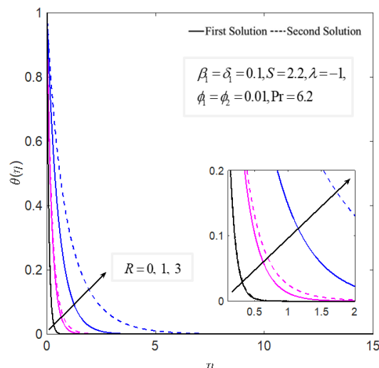
Fig. 7. Temperature profiles \theta(\eta) against R
