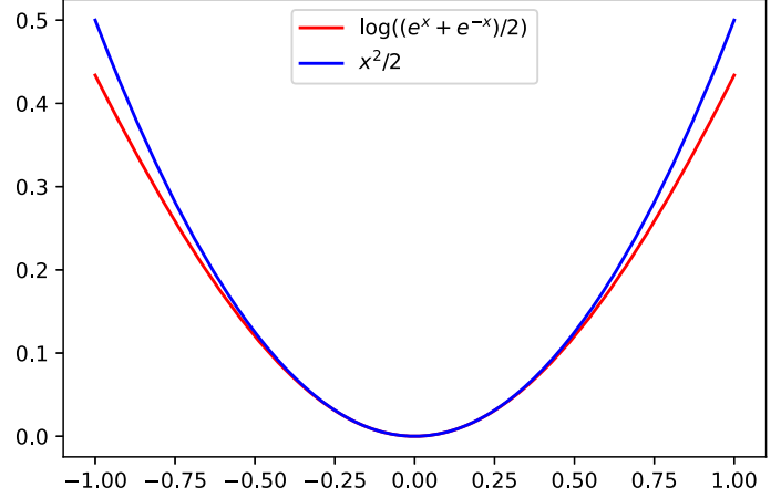
Figure 1: The inequality (4.6) on the log scale.
