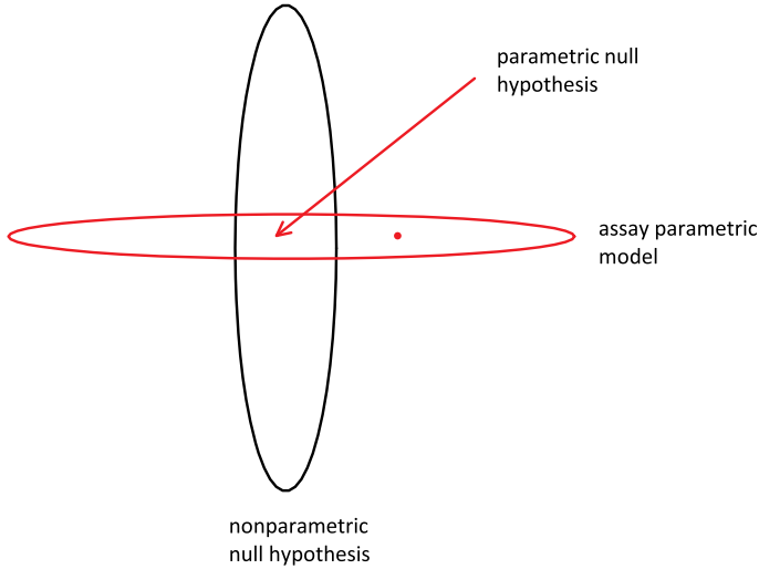
Figure 3: Assaying a non-parametric e-test.
