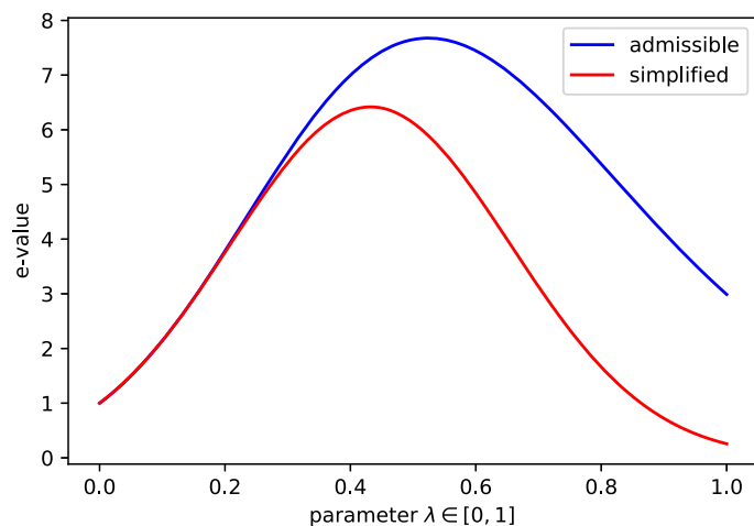
Figure 2: Results for the Fisher-type e-test applied to Darwin’s data.
