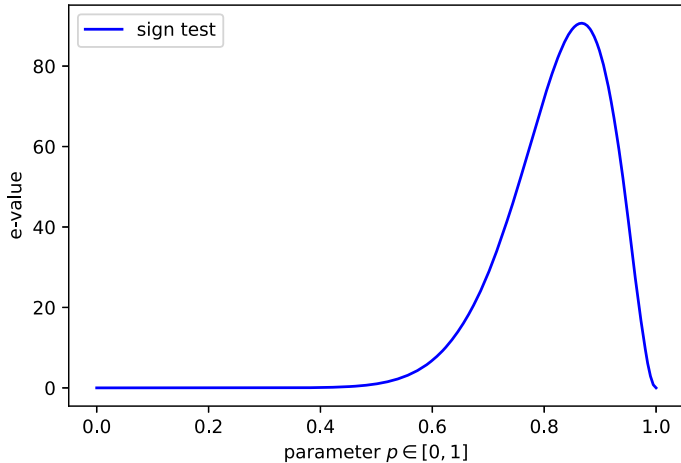
Figure 4: Results for the sign e-test applied to Darwin’s data.
