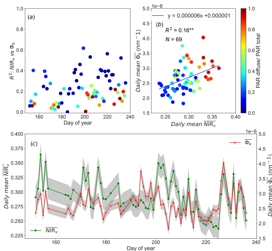
Figure 3. Panel (a) exhibits the inter-daily variations of the coefficient of determination ( R^2 ) of the relationships between the near-infrared reflectance of vegetation index ( \overline{NIR_v} ) and the canopy \Phi_k at instantaneous scale, as a function of the fraction between diffuse and total PAR. Panel (b) presents the seasonal relationship between the daily means \overline{NIR_v} and \overline{\Phi_k} , as a function of the fraction between diffuse and total PAR. And panel (c) shows the seasonal dynamics in \overline{NIR_v} and \overline{\Phi_k} . The shaded area indicates the 95 % confidence interval. The asterisks stand for the statistical significance level (** = P \leq 0.01 ).
