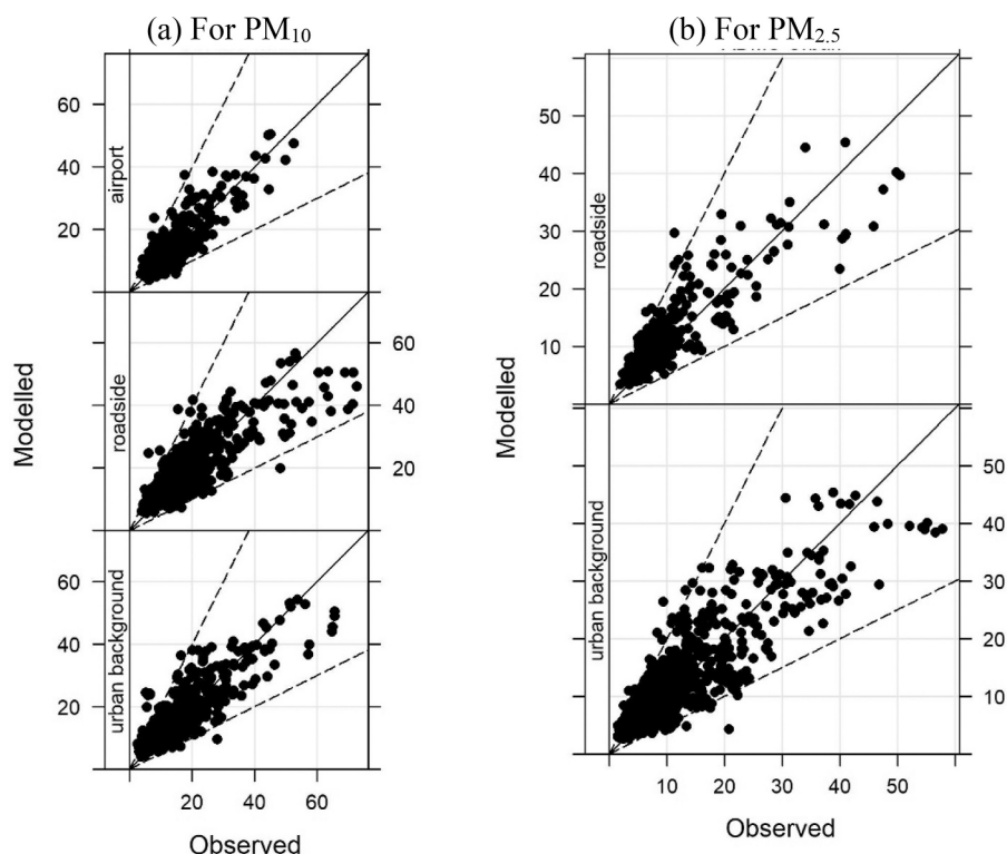
Fig. 4. Scatter plots of daily averages between the modelled and measured data for 3 types of sites (airport, roadside and urban background): (a) for PM 10 (in \mu\text{g m}^{-3} ) and (b) for PM 2.5 (in \mu\text{g m}^{-3} ). These dashed lines represent the slopes of 0.5 and 2 respectively (indicating a factor of 2 between the modelled and measured data).
