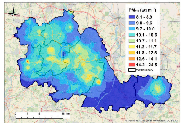
(f) PM 2.5 for Case Re0.9
