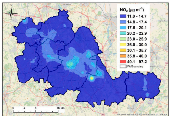
Fig. 6. Annual air quality map of NO 2 (in \mu\text{g m}^{-3} ) at 10 m \times 10 m resolution for (a) Case 2019 BAU, and percentage change (reduction in %) of NO 2 for (b) Case Re0.1, (c) Case Re0.3, (d) Case Re0.5, (e) Case Re0.7, and (f) Case Re0.9, relative to Case 2019 BAU.
