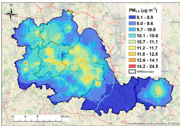
(e) PM 2.5 for Case Re0.7
