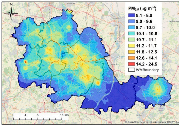
(c) PM 2.5 for Case Re0.3
