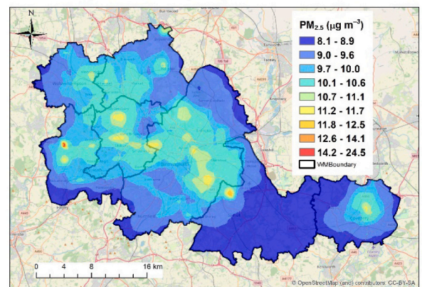
Fig. 7. Annual air quality map of PM 2.5 (in \mu\text{g m}^{-3} ) at 10\text{ m} \times 10\text{ m} resolution for (a) Case 2019 BAU, and percentage change (reduction in %) of PM 2.5 for (b) Case Re0.1, (c) Case Re0.3, (d) Case Re0.5, (e) Case Re0.7, and (f) Case Re0.9, relative to Case 2019 BAU.
