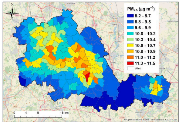
(f) PM 2.5 for Case Re0.9
