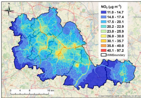
(c) NO 2 for Case Re0.3
