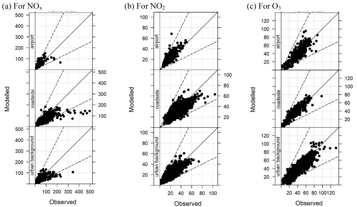
Fig. 3. Scatter plots of daily averages between the modelled and measured data for 3 types of sites (airport, roadside and urban background): (a) for \text{NO}_x (in \mu\text{g m}^{-3} ), (b) for \text{NO}_2 (in \mu\text{g m}^{-3} ) and (c) for \text{O}_3 (in \mu\text{g m}^{-3} ) for the baseline year of 2019. These dashed lines represent the slopes of 0.5 and 2 respectively (indicating a factor of 2 between the modelled and measured data).
