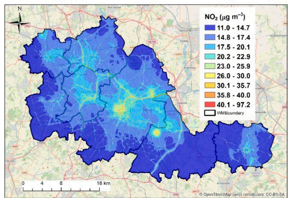
(f) NO 2 for Case Re0.9
