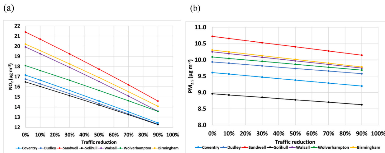
Fig. 10. (a)NO 2 and (b)PM 2.5 at local authority levels (averages calculated based on 10 m × 10 m resolution maps). “0%” represents the 2019 baseline BAU case. Traffic reductions of “10%”, “30%”, “50%”, “70%”, and “90%” represent Case Re0.1, Case Re0.3, Case Re0.5, Case Re0.7 and Case Re0.9, respectively.
