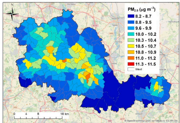
Fig. 9. Annual air quality map of PM 2.5 (in \mu\text{g m}^{-3} ) at the ward level for (a) Case 2019 BAU, and percentage change (reduction in %) of PM 2.5 for (b) Case Re0.1, (c) Case Re0.3, (d) Case Re0.5, (e) Case Re0.7, and (f) Case Re0.9, relative to Case 2019 BAU.
