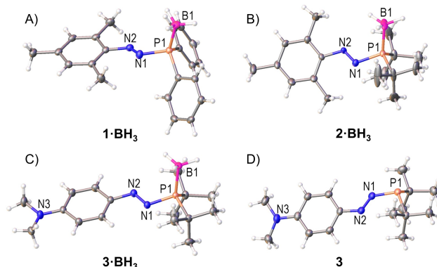
Figure 2. Single crystal structures of \mathbf{1}\cdot\text{BH}_3 (A); \mathbf{2}\cdot\text{BH}_3 (B); \mathbf{3}\cdot\text{BH}_3 (C); \mathbf{3} (D). Selected bond distances (Å) and angles ( ^\circ ): \mathbf{1}\cdot\text{BH}_3 \text{N1}-\text{N2} 1.2504(14), \text{N1}-\text{P1} 1.7565(10), \text{P1}-\text{N1}-\text{N2} 115.00(8); \mathbf{2}\cdot\text{BH}_3 \text{N1}-\text{N2} 1.226(6), \text{N1}-\text{P1} 1.769(5), \text{P1}-\text{N1}-\text{N2} 113.5(4); \mathbf{3}\cdot\text{BH}_3 \text{N1}-\text{N2} 1.2681(17), \text{N1}-\text{P1} 1.7380(12), \text{P1}-\text{N1}-\text{N2} 114.33(10); \mathbf{3} \text{N1}-\text{N2} 1.258(3), \text{N1}-\text{P1} 1.7494(18), \text{P1}-\text{N1}-\text{N2} 119.34(14). Thermal ellipsoids were drawn at the 50% probability level. [14]
