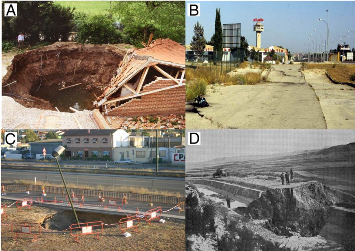
Figure 1. A: Building severely damaged by a collapse sinkhole occurred on April 23, 1997 over Permian gypsum in Ripon (NE England) photo copyright BGS, NERC. B: Bending subsidence affecting a service road located between the N-232 motorway and the Pikolín factory, on the outskirts of Zaragoza city (river terrace in the Ebro Valley, NE Spain). This stretch of the road is located over the artificially-filled sinkholes shown in figure 3. Photograph taken in June, 1996. C: Collapse sinkhole formed next to the N-232 motorway during the night of May 23, 2006 (Ebro River terrace close to Zaragoza city). The three stacked artificial fills exposed in the overhanging margins suggest that this sinkhole resulted from the reactivation of a previously existing karstic depression. Photograph taken 8 days after the subsidence event. D: Collapse sinkhole that occurred in 1954 in the La Violada Canal (Ebro Tertiary Basin, NE Spain). Photograph taken from Llamas (1962).
