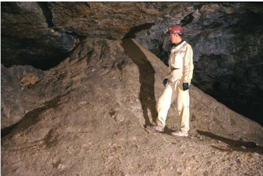
Figure 5. Fresh debris cone in the Mylinki Cave (gypsum karst of western Ukraine) generated by the active upward propagation of a joint-controlled cavity. This accumulation allows identifying the probable location of a future sinkhole. Photograph taken in May 1999, copyright BGS, NERC.
