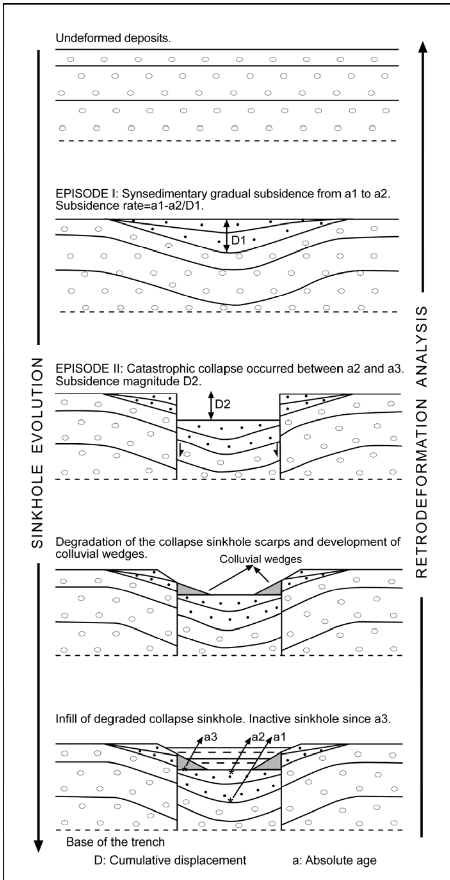
Figure 6. Theoretical example of the application of retrodeformation analysis and absolute dating techniques to the investigation of sinkholes in a mantled karst setting.
