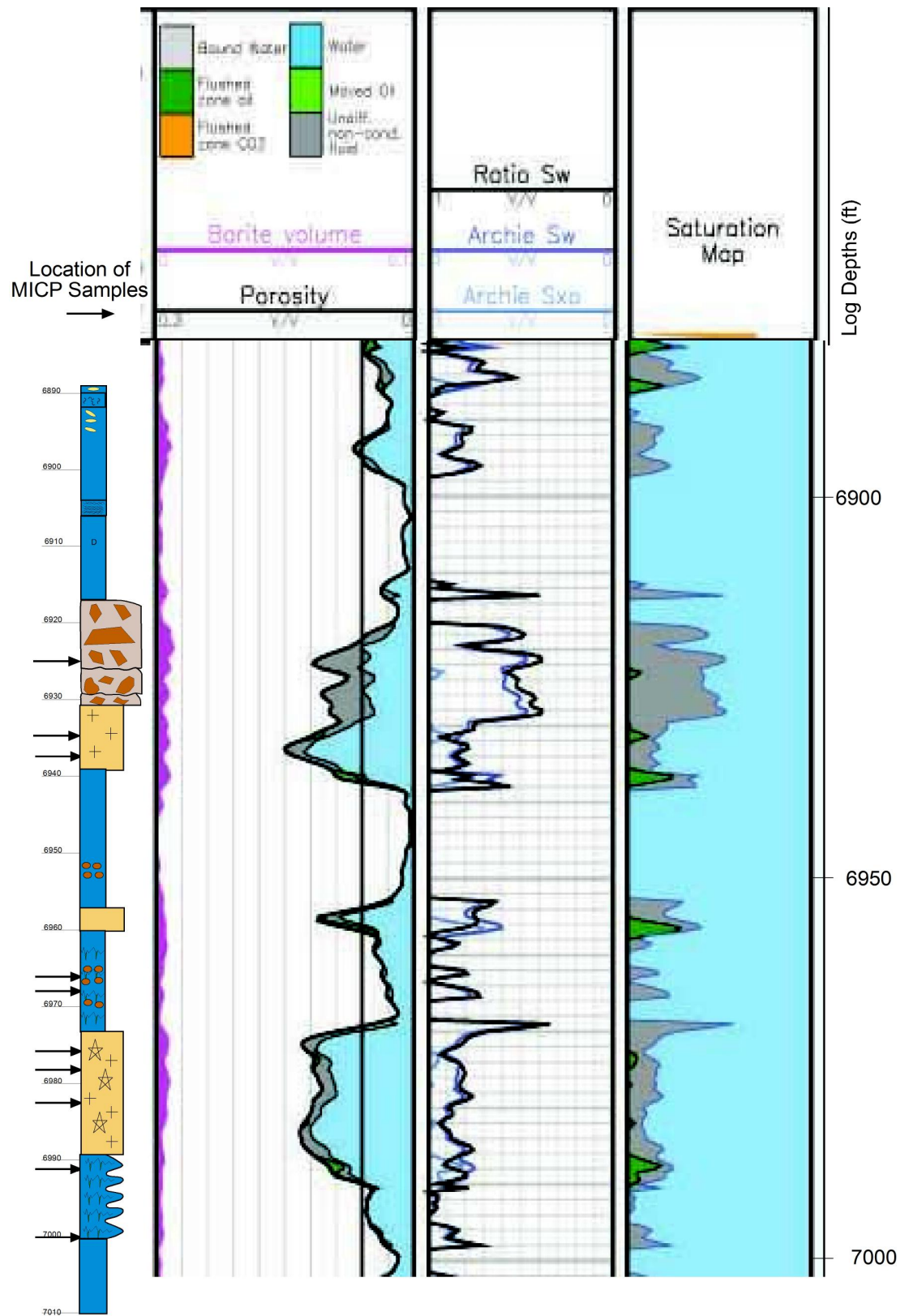
Figure 5. Log-calculated water saturation by Jeff Kane, Kinder Morgan, and core description showing an abrupt increase in Sw within the upper porous zone.
