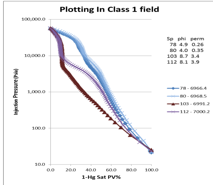
Figure 3. Mercury injection capillary pressure curves for class 3, fractured and moldic wackestones that plot in the class 1 field.
