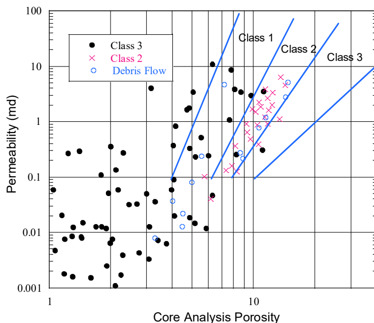
Figure 1. Cross-plot of porosity and permeability showing petrophysical class fields and rock fabric petrophysical class of samples.
