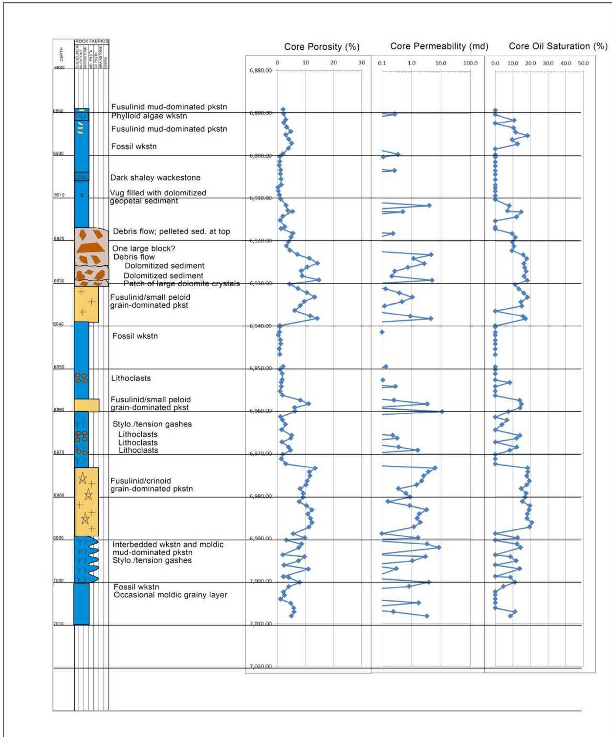
Figure 2. Geologic core description and plot of core analysis data.
