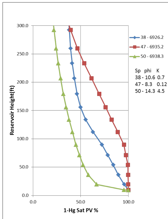
Figure 7. MICP curves for upper porous interval converted to reservoir height. Sample 38 at 6,926.2 ft depth is from the debris flow.
