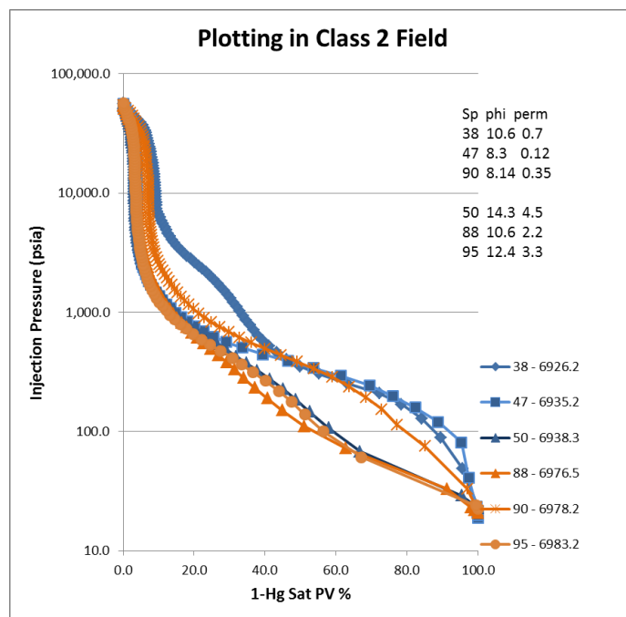
Figure 4. Mercury injection capillary pressure curves for class 2, grain-dominated packstones that plot in the class 2 field.
