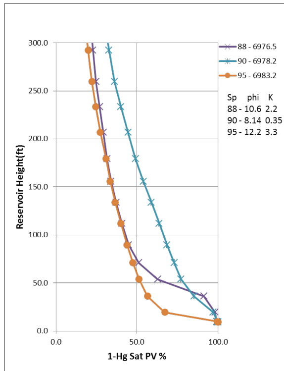
Figure 6. MICP curves for lower porous interval converted to reservoir height.
