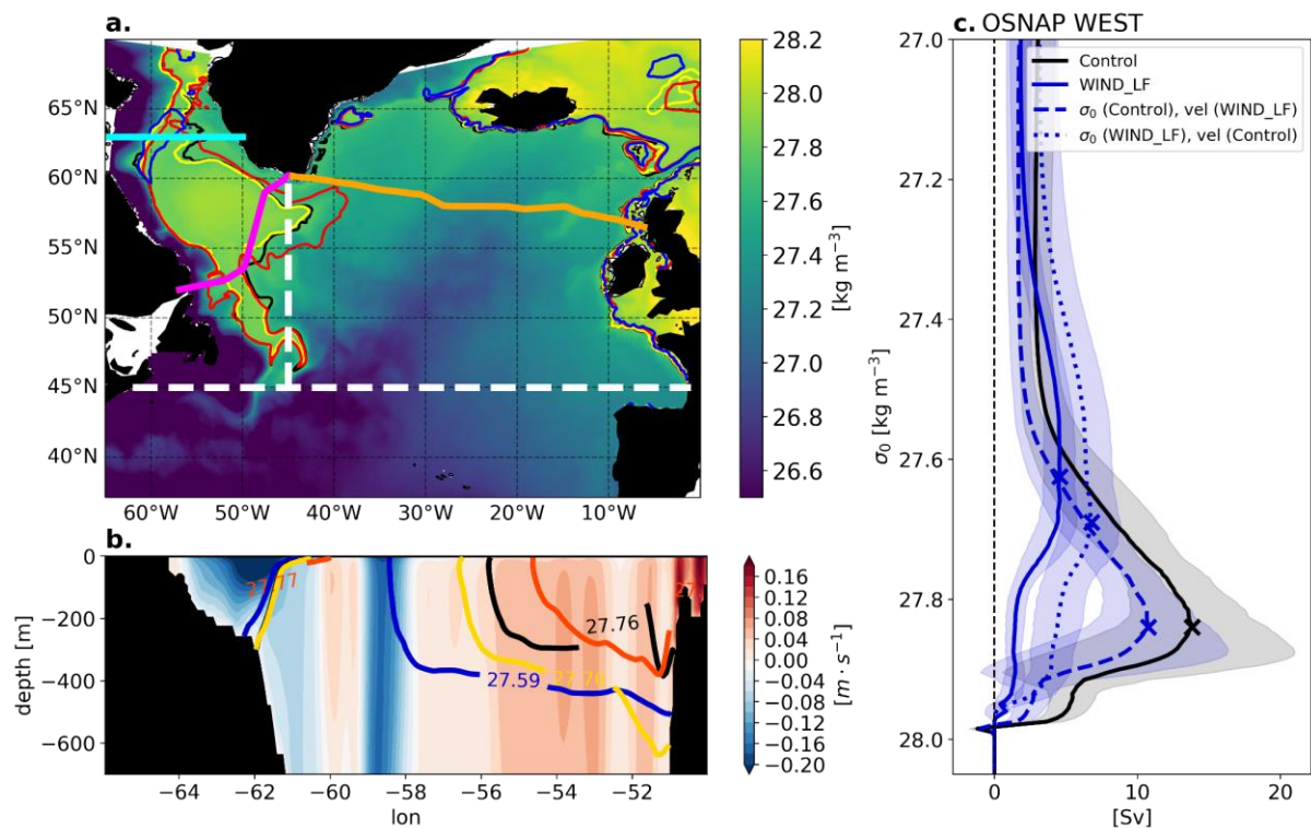
Fig. 11. Mean surface potential density ( \sigma_0 ) in winter (January-March) for the control experiment during years 11-15 (a). Contour lines correspond to isopycnals of maximum overturning across OSNAP line (refer to Figure 10) in the control experiment (black, \sigma_0=27.76 kg/m 3 ), WIND_LF (blue, \sigma_0=27.59 kg/m 3 ), WIND_LF_SYNOPT (yellow, \sigma_0=27.76 kg/m 3 ), and WIND_SCALED_LF (red, \sigma_0=27.77 kg/m 3 ). Magenta and orange lines show the location of
