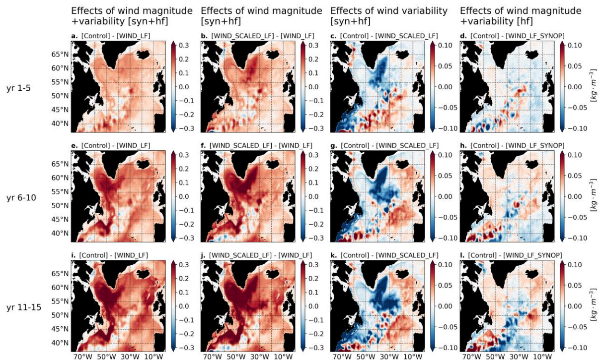
Fig. 6. Same as Fig. 4, but for mean potential density ( \sigma_0 ) in the upper 500 m.
