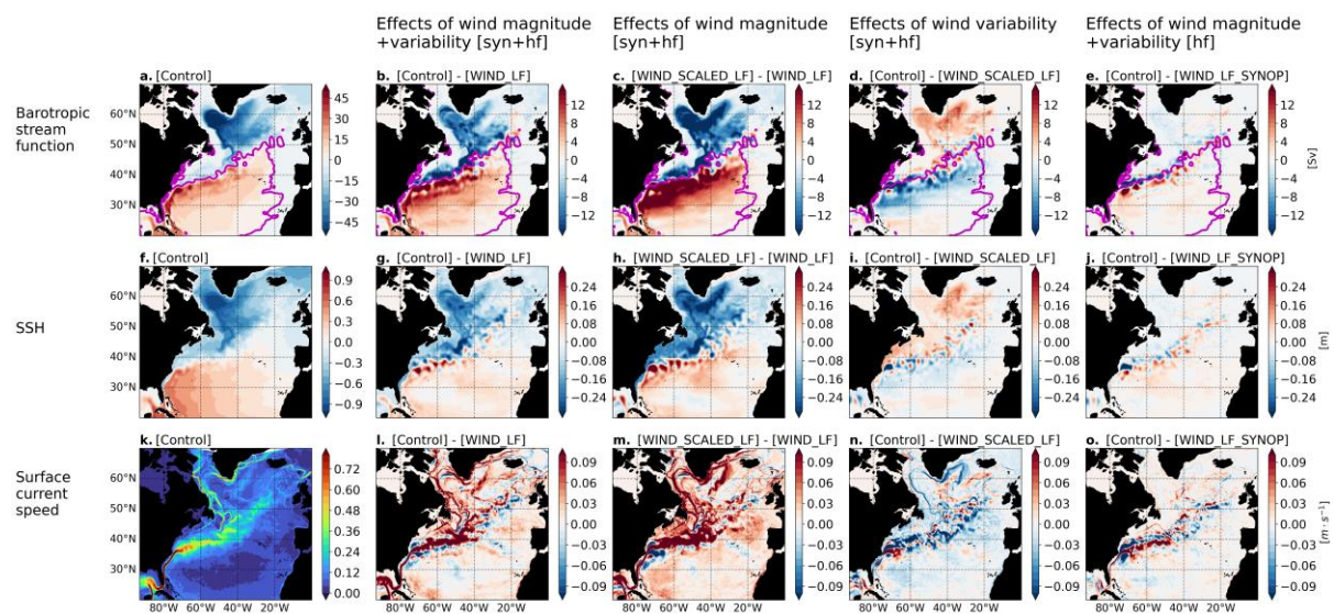
Fig. 7. Barotropic stream function (a), sea surface height (f), and surface current speed (k), averaged over years 11-15 in control experiment. Second column (b, g, l) shows the differences between control and experiment forced by low-frequency winds (highlighting the effect of wind magnitude and variability associated with synoptic and higher frequency winds ); third column (c, h, m) shows show the differences between the experiments forced by scaled versus non-scaled low-frequency winds (highlighting the effect of wind magnitude associated with synoptic and higher frequency winds ); fourth column (d, i, n) shows the differences between control and experiment forced by scaled low-frequency winds (highlighting the effect of wind variability associated with synoptic and higher frequency winds ); fifth column (e, j, o) show the differences between control and experiment forced by low-frequency and synoptic winds (highlighting the effect of wind magnitude and variability associated with synoptic and higher frequency winds ). Magenta contour lines (a-e) show the zero line of the barotropic stream function in the control experiment, averaged over years 11-15.
