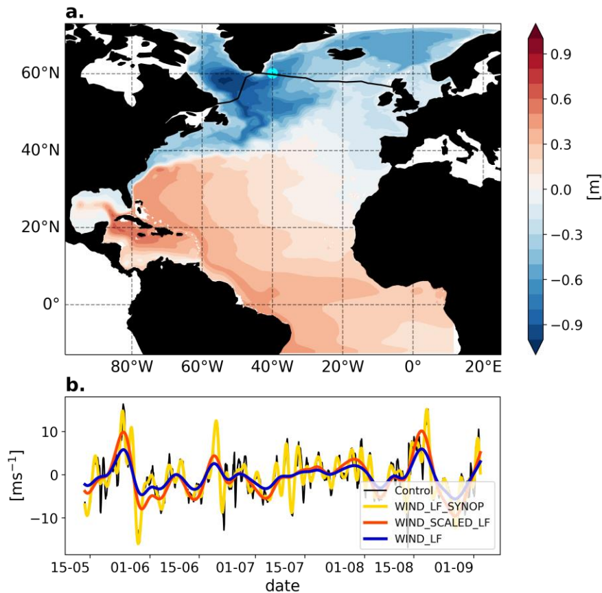
Fig. 1. Mean relative dynamic sea surface height during the winter season (January–March) of years 11–15 over the regional domain of the MITgcm (a); 4 months’ time series of 10-m zonal wind speed (b) in the location shown with the cyan dot in panel (a) in the Irminger Sea. The time series comprises JRA55-do reanalysis data used as forcing for the control experiment (black), along with filtered low-frequency winds (blue), low-frequency plus synoptic winds (yellow), and scaled low-frequency winds (red). Black line in panel (a) shows the position of the observational OSNAP array.
