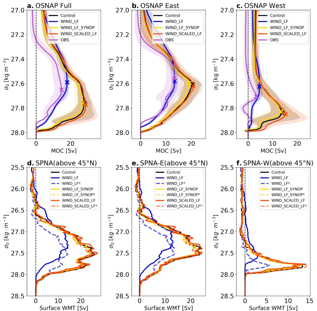
Fig. 10. Meridional overturning stream function in density space across the full OSNAP array (a), OSNAP East (b) and OSNAP West (c) sections, from control experiment (black) and sensitivity tests (blue, yellow, red) averaged over years 11-15 and compared to OSNAP observations (purple) averaged over August 2014 - May 2018; standard deviation for each density class is shown in shading. The location of the OSNAP lines is illustrated in Fig. 11a. The lower panels display surface water mass transformations calculated within the region north of 45°N (d), further separated into the regions east of 45°W (e) and west of 45°W (f) shown with the dashed lines in Fig. 11a.
