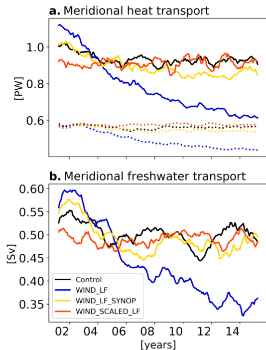
Fig. 8. Time series of meridional heat (a) and freshwater (b) transport across 40°N in control experiment (black) and sensitivity tests: experiment forced by low-frequency winds (blue), experiment forced by low-frequency + synoptic winds (yellow), and experiment forced by scaled low-frequency winds (red). Dotted lines in panel (a) show meridional heat transports across 60°N.
