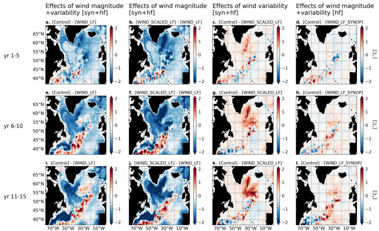
Fig. 4. Differences in mean potential temperature in the upper 500 m between the control run and sensitivity tests, averaged over years 1-5 (upper row; a-d), years 6-10 (middle row; e-h), and years 11-15 (lower row; i-l). First column (a, e, i) shows the differences between control and experiment forced by low-frequency winds (highlighting the effect of wind magnitude and variability associated with synoptic and higher frequency winds ); second column (b, f, j) shows the differences between the experiment forced by scaled versus non-scaled low-frequency winds (highlighting the effect of wind magnitude associated with synoptic and higher frequency winds ); third column (c, g, k) shows the differences between control and experiment forced by scaled low-frequency winds (highlighting the effect of wind variability associated with synoptic and higher frequency winds ); and fourth column (d, h, l) shows the differences between control and experiment forced by low-frequency and synoptic winds (highlighting the effect of wind magnitude and variability associated with synoptic and higher frequency winds ).
