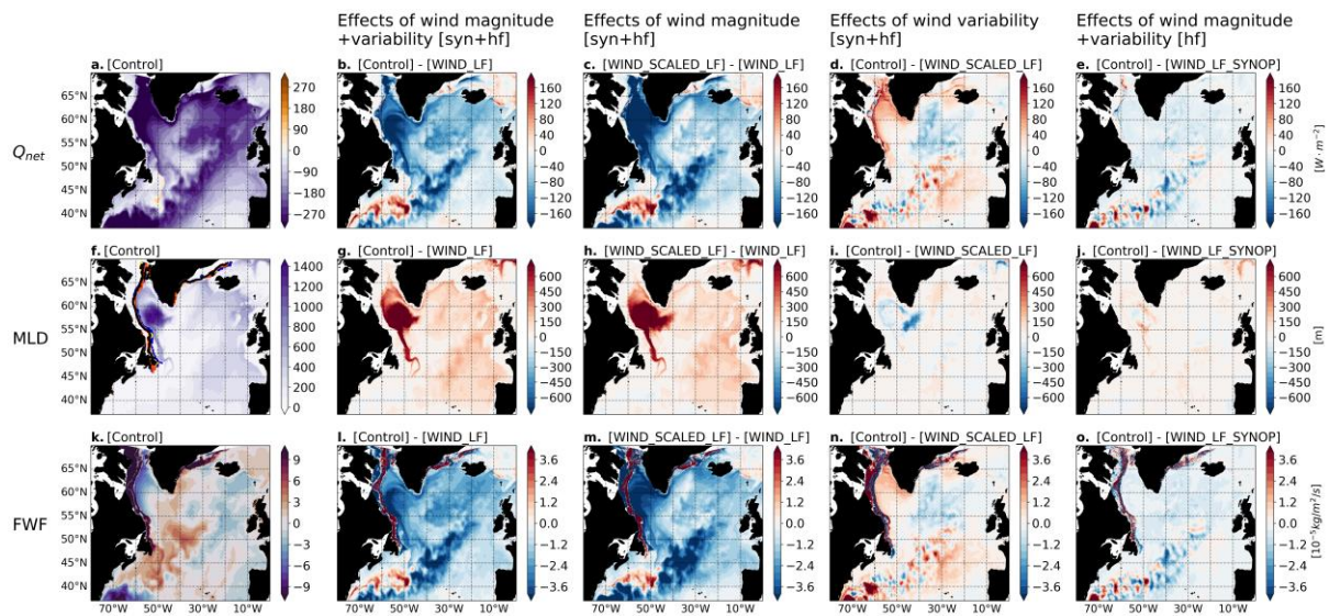
Fig. 3. Net heat flux into the ocean ( Q_{net} ; a) in winter (January-March), mean mixed layer depth (MLD) in March (f) and freshwater flux into the ocean in winter (k; January-March) in years 11-15 in control experiment. Positive values of net heat flux correspond to flux into the ocean; positive values of freshwater flux correspond to decrease in salinity. Coloured contours on panel (e) show 15% concentration of the sea ice in control experiment (black), experiment forced by low-frequency winds (blue), low-frequency plus synoptic winds (yellow), and scaled low-frequency winds (red). Second column (b, g, l) shows the differences between control and experiment forced by low-frequency winds (highlighting the effect of wind magnitude and variability associated with synoptic and higher frequency winds ); third column (c, h, m) shows the differences between the experiments forced by scaled versus non-scaled low-frequency winds (highlighting the effect of wind magnitude associated with synoptic and higher frequency winds ); fourth column (d, i, n) shows the differences between control and experiment forced by scaled low-frequency winds (highlighting the effect of wind variability associated with synoptic and higher frequency winds ); the fifth column (e, j, o) show the differences between control and experiment forced by low-frequency and synoptic winds (highlighting the effect of wind magnitude and variability associated with synoptic and higher frequency winds ).
