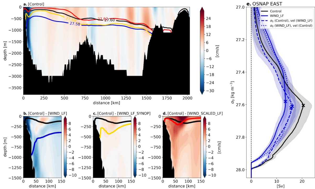
Fig. 12. Mean velocity across the OSNAP-East line (shown in Fig. 11 with solid orange line) in the control experiment (a), contours show annual mean positions of isopycnals of maximal overturning across OSNAP-East in the control experiment (black), WIND_LF (blue), WIND_LF_SYNOPT (yellow), WIND_SCALED_LF (red); differences between control and experiment forced by low-frequency winds (b), the differences between control and experiment forced by low-frequency and synoptic winds (c), the differences between control and experiment forced by scaled low-frequency winds (d). Panel e shows meridional overturning circulation in density space ( MOC_{\sigma_0} ) across OSNAP-East (purple line in Fig. 11a): dashed blue line shows MOC_{\sigma_0} computed using densities from control experiment and velocities from WIND_LF; dotted blue line shows MOC_{\sigma_0} computed using densities from WIND_LF experiment and velocities from control experiment.
