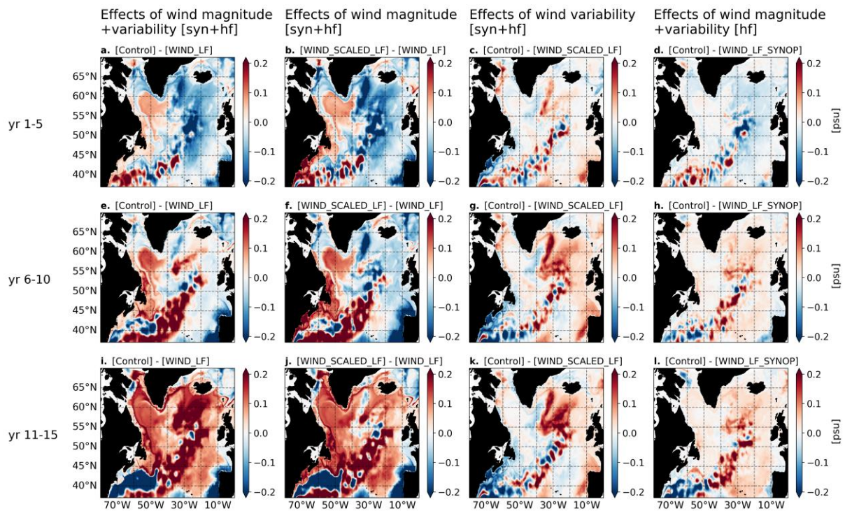
Fig. 5. Same as Fig. 4, but for salinity in the upper 500 m.
