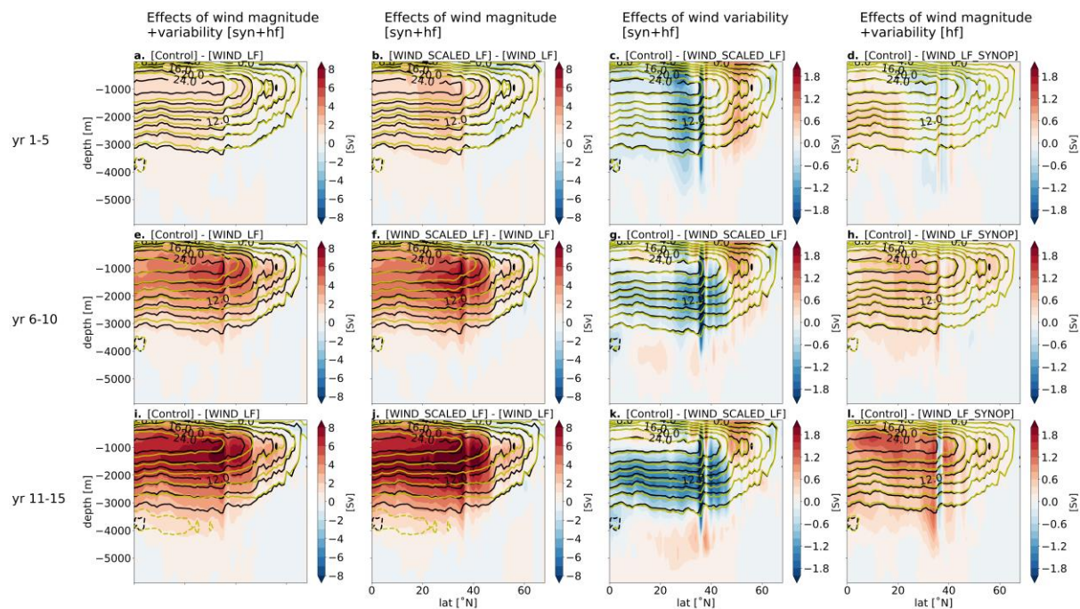
Fig. 9. Differences in meridional overturning stream function in depth space between the control run and sensitivity tests averaged over years 1-5 (upper row; a-d), years 6-10 (middle row; e-h), and years 11-15 (lower row; i-l); black contours show the meridional overturning streamfunction in the control run, and yellow contours in each of the sensitivity experiments. First column (a,e,i) shows the differences between control and experiment forced by low-frequency winds (highlighting the effect of wind magnitude and variability associated with synoptic and higher frequency winds ); second column (b, f, j) shows the differences between the experiments forced by scaled versus non-scaled low-frequency winds
