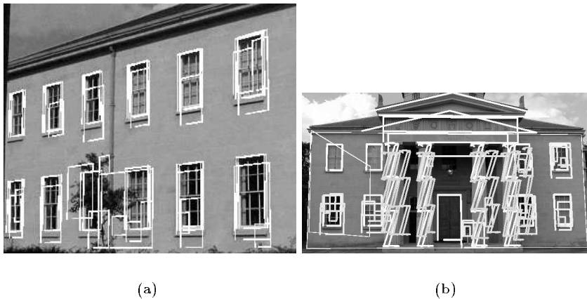
Figure 9: Collection of shapes whose likelihood ratio of being a window to not being a window is high. The zig-zag shapes correspond to columns.
