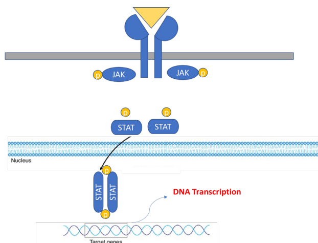
Figure 5. JAK-STAT signaling pathway illustration. Notes: Particular ligands bind to their associated receptors to activate the JAK component. To activate its kinase function, JAK phosphorylates its tyrosine component, which then phosphorylates the STAT component. STATs that have been activated go into the nucleus to encourage DNA transcription. JAK: Janus kinase, and STAT: signal transducer and activator of transcription.
