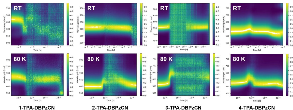
Figure 6: Normalized time-resolved emission spectra (contour plots) for all isomers in 0.1 w/w% zeonex films ( \lambda_{\text{exc}} = 355 nm) at room temperature (top row) and 80 K (bottom row).
