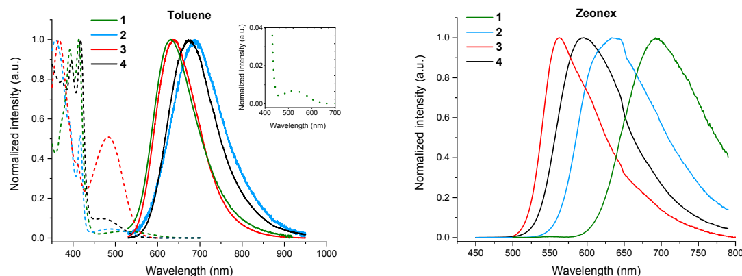
Figure 5: Normalized steady-state absorption (dashed lines) and emission spectra (solid lines) for all four isomers in 10^{-5} M toluene solution (left, \lambda_{\text{exc}} = 440 nm) and emission spectra for 0.1 w/w% zeonex solid films (right, \lambda_{\text{exc}} = 440 nm). Graph inset (left) shows the magnified absorption spectrum of 1-TPA-DBPzCN , revealing a weak CT absorption band. The inflexion around 650 nm in the emission spectra of all four isomers in zeonex film (right) is attributed to the onset of significant instrument-specific intensity correction at longer wavelengths.
