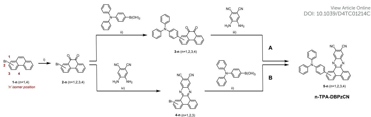
Scheme 1: Synthesis protocol for 1-TPA-DBPzCN , 2-TPA-DBPzCN , 3-TPA-DBPzCN , and 4-TPA-DBPzCN : (i) \text{CrO}_3 , glacial acetic acid, reflux, 2 h; (ii) \text{Pd}(\text{PPh}_3)_4 , \text{Na}_2\text{CO}_3 , toluene, water, reflux, 24 h; (iii) \text{HCl} (37%), EtOH, THF, 40 °C, 24 h; (iv) glacial acetic acid, reflux, 24 h.
