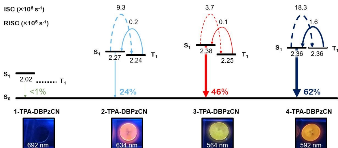
Figure 8: Schematic overview of the main emission characteristics of 1-TPA-DBPzCN (green), 2-TPA-DBPzCN (blue), 3-TPA-DBPzCN (red), and 4-TPA-DBPzCN (black) in 0.1 w/w% zeonex films. The relative positions of the first excited singlet and triplet states are shown according to their experimentally determined energies (in eV), with the exception of the triplet state of 1-TPA-DBPzCN . The corresponding CT (black) or LE (white) character of the excited state is also indicated. The photoluminescence quantum yields are expressed in percentages.
