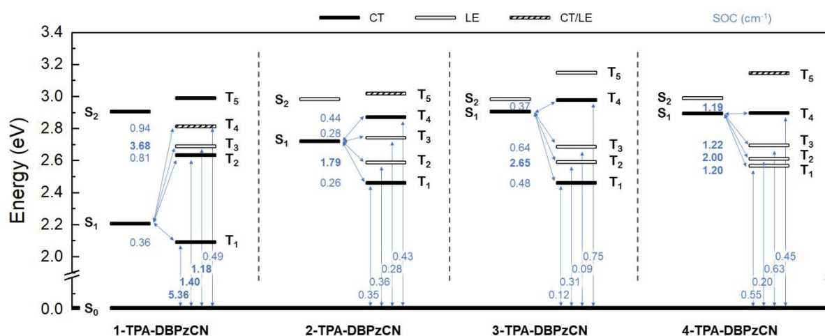
Figure 4: Schematic overview of the excited state energy levels (in eV) of all four isomers with their corresponding CT (black), LE (white), and mixed CT/LE (dashed) character as obtained through TDDFT calculations. Relevant S_0 - T_x and S_1 - T_x ( x = 1-5 ) couplings and SOC values are shown in blue (SOC values > 1 \text{ cm}^{-1} in bold).
