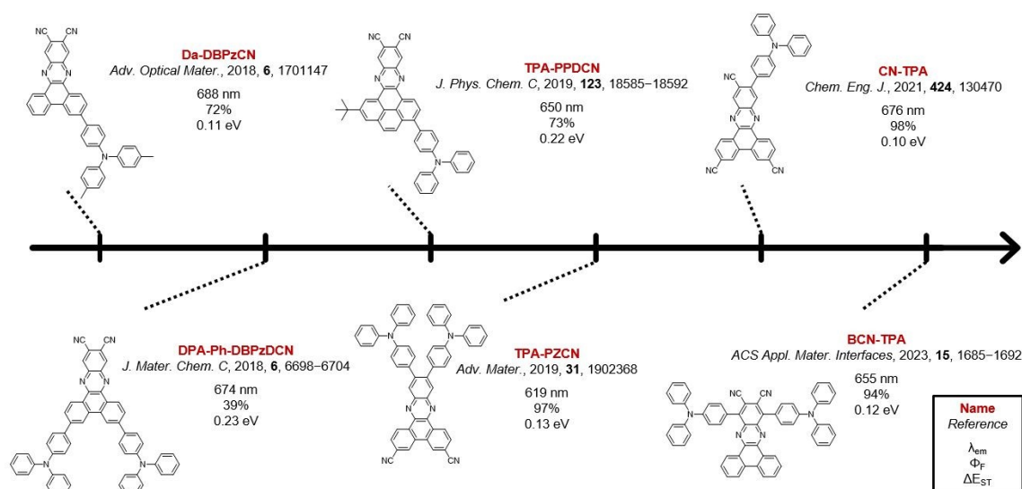
Figure 1: Examples of reported red TADF emitters based on the DBPzCN acceptor. The main photophysical characteristics (emission wavelength, fluorescence quantum yield, and singlet-triplet energy gap) are given for the materials in doped films.
