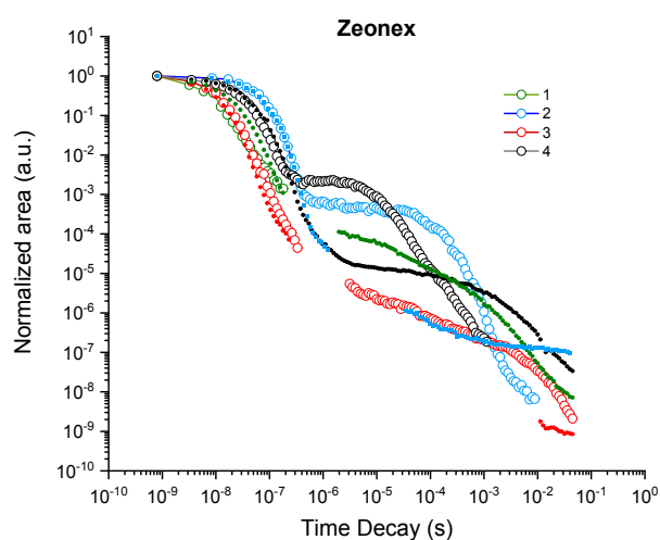
Figure 7: Total emission decay (calculated via the integrated area under the emission curve) for 1-TPA-DBPzCN (green), 2-TPA-DBPzCN (blue), 3-TPA-DBPzCN (red), and 4-TPA-DBPzCN (black) at room temperature (open circles) and 80 K (closed circles). Data points with signal below the noise baseline have been omitted from the figure.
