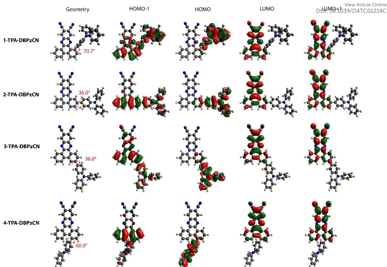
Figure 3: Optimized molecular geometries and orbital spatial distributions (LUMO+1, LUMO, HOMO, and HOMO-1) for 1-TPA-DBPzCN , 2-TPA-DBPzCN , 3-TPA-DBPzCN , and 4-TPA-DBPzCN . Values of dihedral angles are given in red. Isocontour values of 0.02 (a.u.) were used for all orbitals.
