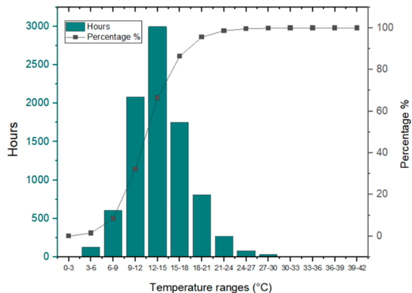
Figure 8. San Francisco frequency of ambient air temperature.
