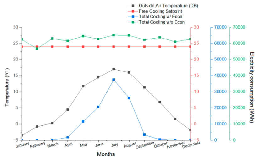
Figure 12. Stockholm outdoor air temperature cooling electricity impact (economiser vs. no economiser).
