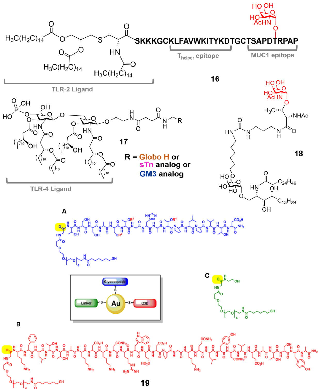
Fig. 14. Structures of: 16 glycoconjugate vaccine containing tandem repeating unit of MUC-1 conjugated to the TLR2 ligand [294]; 17 glycoconjugate vaccine containing a TACA antigen (sTn, GM3, Globo-H) conjugated to a TLR-4 ligand [300–302], 18 a synthetic Tn antigen-glycolipid containing an \alpha -GalCer residue [305]; 19 Au nanoconstructs, containing the TF disaccharide antigen instead of the Tn antigen. Figure of compound 19 reproduced from Ref. [308]. Copyright 2012, American Chemical Society.
