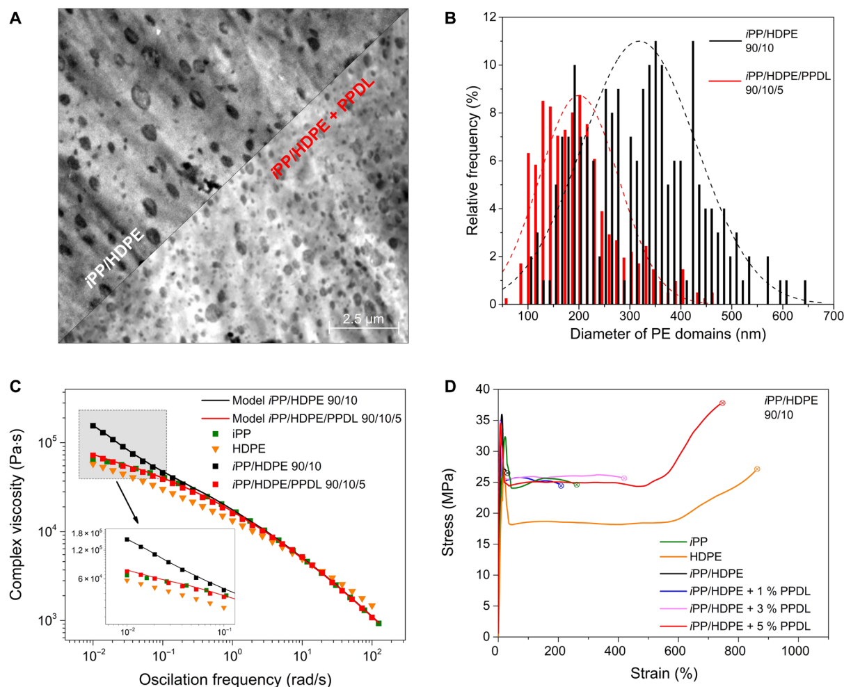
Fig. 3. Morphology and performance analysis of i PP/HDPE 90/10 w/w blends. TEM image of the i PP/HDPE 90/10 w/w blend and i PP/HDPE/PPDL 90/10/5 w/w blend (A). The compatibilizing effect of PPDL visualized by HDPE-dispersed phase size determination in i PP/HDPE and i PP/HDPE/PPDL blends using TEM (B). Measured (symbols) and calculated (line) complex viscosity ( \eta^* ) of i PP, HDPE, uncompatibilized i PP/HDPE 90/10 blend, and compatible i PP/HDPE/PPDL 90/10/5 composition. Samples were tested under oscillation frequency ( \omega ) at a constant temperature of 190°C (C). Static mechanical properties measurements of the compatibilized i PP/HDPE/PPDL blend, the uncompatibilized i PP/HDPE blend, and i PP, HDPE, and PPDL reference materials (D).
