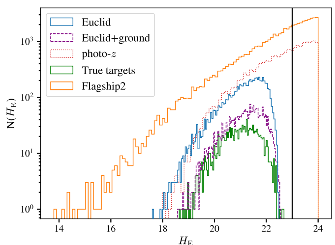
Fig. 9. H_E -band number counts for samples built from the Flagship2 catalogue. The samples selected with the neural network classifier, using Euclid photometry only or combined with ground-based photometry are shown, respectively, by the blue-solid and magenta-dashed histograms. As indicated by the legend, the red-dotted histogram corresponds to a sample selected in redshift only, using Euclid photometric redshifts. The counts for the full Flagship2 catalogue and the true target sample are also shown for reference, by the orange and green histograms. Note how the distribution of the true targets (green histogram) dies off at magnitudes fainter than H_E \approx 22.5 . The targets in the EL-COSMOS catalogue extend to fainter flux.
