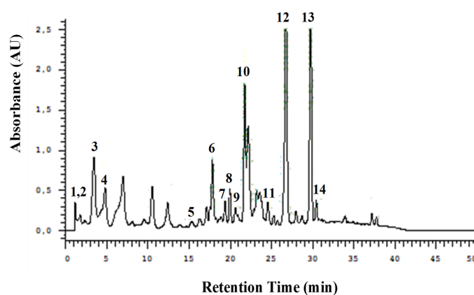
Fig. 1. : Chemical characterization of PRO (from BRPX propolis) dried ethanolic extract analyzed by High-performance liquid chromatography (HPLC) and monitored at wavelengths of 280 and 320 nm. Peaks are: moncaffeoylquinic acid (1), caffeic acid (2), p-coumaric acid (3), 3,5-di-O-caffeoylquinic acid (4), kaempferol (5), 2,2-dimethyl-2 H-1-benzopyranpropenoic acid (culifolin) (6), 3-prenyl-4-hydroxycinnamic acid (drupanin) (7), 4-hydroxy-3(E)-(4-hydroxy-3-methyl-2-butenyl)–5-prenylcinnamic acid (8), 3-prenyl-4-(2-methylpropionyloxy)-cinnamic acid (9), kaempferide (10), 3-hydroxy-2,2-dimethyl-8-prenyl-2 H-1-benzopyran-6-propenoic acid (11), 3,5-diprenyl-4-hydroxycinnamic acid, Artepillin-C (12), 2,2-dimethyl-8-prenyl-2 H-1-benzopyran-6-propenoic acid (13) and 3-prenyl-4-dihydrocinnamoyloxy cinnamic acid (14). AU corresponds to Absorbance Units.
