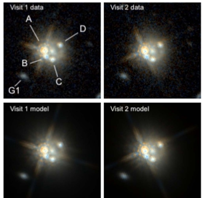
Figure 16. HST WFC3/IR F125W and F160W color-combined images of W2M J1042+1641 over two visits, along with output from a morphological analysis with hostlens , as in Figure 2, but with a “free SIE+ \gamma ” model.
