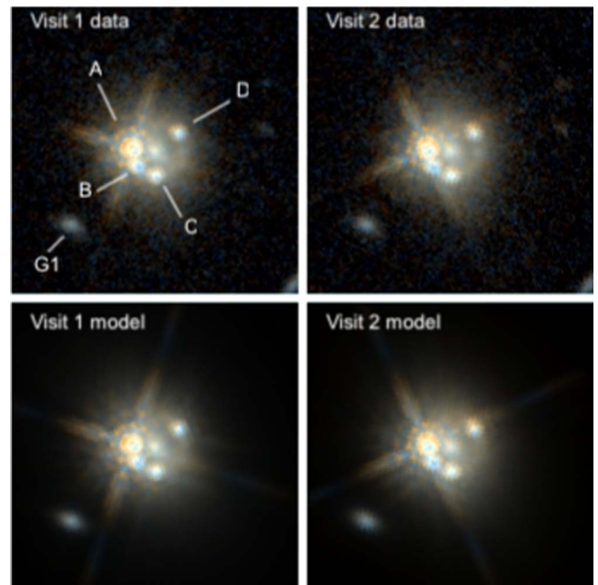
Figure 2. HST WFC3/IR F125W and F160W color-combined images of W2M J1042+1641 over two visits, along with output from a morphological analysis with hostlens . The top row shows the observed, drizzled image. The second row shows the best-fit model consisting of four PSFs, Sérsic profiles for the lensing galaxy (located in between the four PSFs) and G1, and the Einstein ring image of the source host. The modeled components are labeled and referenced in the text. The images are oriented with north pointing up and east to the left, although the two visits were each taken rotated by 47^\circ 2' with respect to each other. The scale is 10'' \times 10'' . Left: visit 1, UT 2017 February 26. Right: visit 2, UT 2017 May 7.
