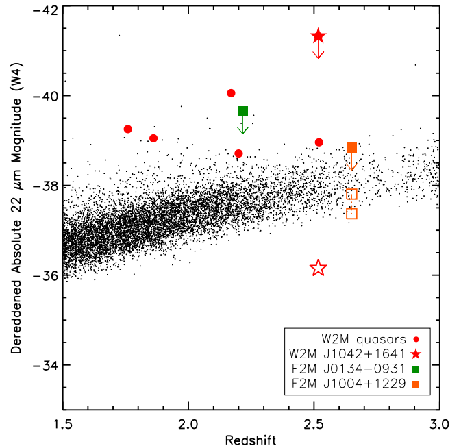
Figure 15. Absolute magnitude at 22 \mu\text{m} in the observed frame, from WISE, for the sample of red QSOs in the W2M survey. The observed luminosity of W2M J1042+1641 is indicated by a star, with a downward-pointing arrow pointing toward its demagnified intrinsic luminosity (using \mu = 117 ). This figure indicates that W2M J1042+1641 is a reddened QSO drawn from a population of sources that is not accessible to the wide-area QSO samples currently being studied. We show, for comparison, the observed and magnification-corrected luminosities of the other high-redshift lensed F2M red quasars discussed in the text, using only an upper limit for F2M J0134–0931 (see text) and the luminosity range for F2M J1004+1229 corresponding to magnification 3.15^{+0.71}_{-0.55} .
