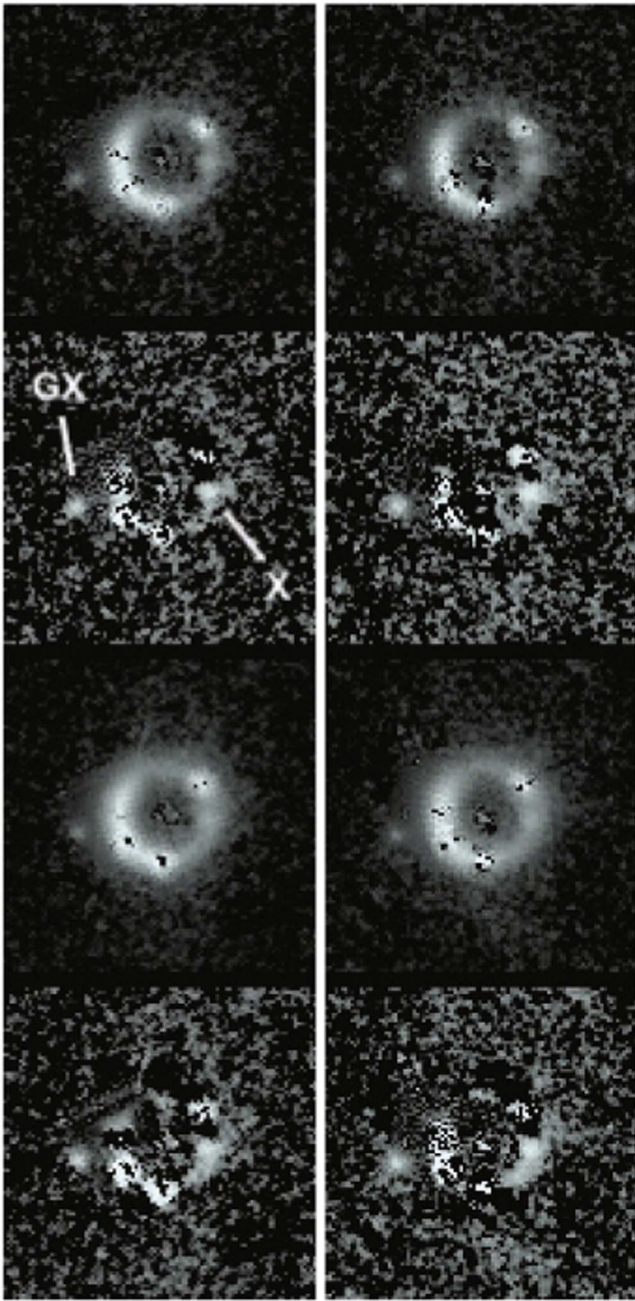
Figure 3. HST residual images of W2M J1042+1641 over two visits, after subtracting the best-fit morphological models determined by hostlens shown in the bottom panel of Figure 2. The top row shows the F125W image with the PSFs and Sérsic profiles subtracted, revealing a clear Einstein ring made up of the lensed QSO’s host galaxy light. The second row shows the full residuals of the same fitted model for the F125W image. The third and fourth rows show the same but for F160W. The labeled components are the nearby object (GX), which we consider as a galaxy perturber associated with the lensing galaxy in our modeling, and a source that is likely associated with the QSO host galaxy (X). The images are scaled to 6'' \times 6'' and oriented to match those in Figure 2. Left: visit 1, UT 2017 February 26. Right: visit 2, UT 2017 May 7.
