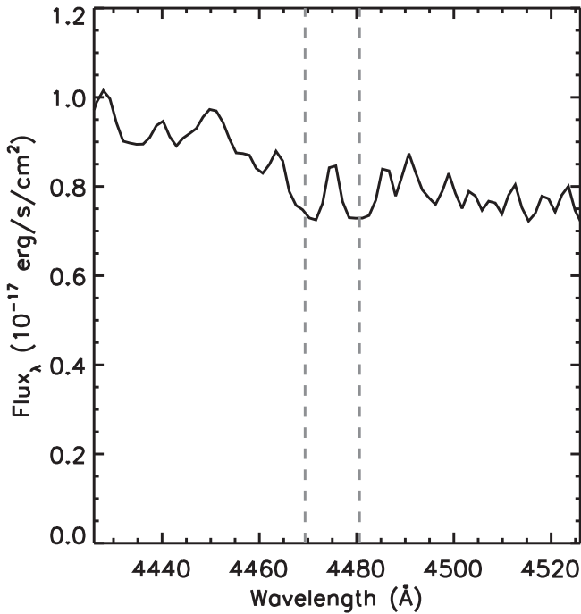
Figure 4. We identify a Mg II \lambda\lambda 2796, 2803 absorption feature, marked by dashed vertical gray lines, at a redshift of z = 0.5985 .
