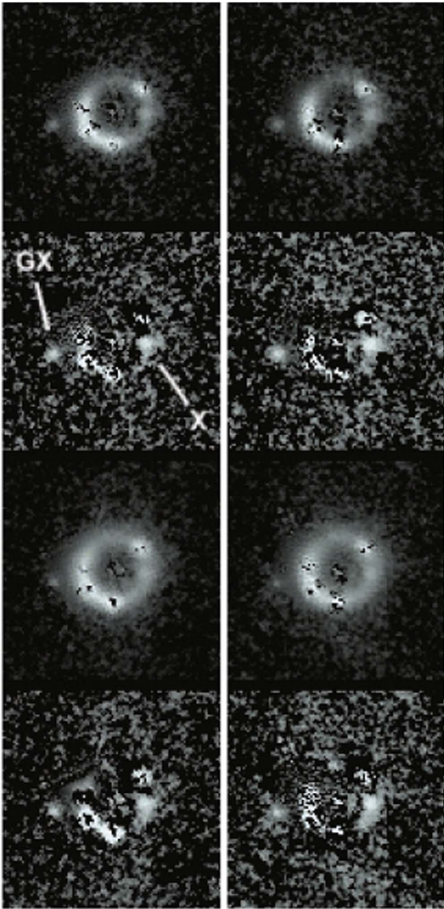
Figure 17. HST Residual images of W2M J1042+1641 over two visits, after subtracting the best-fit morphological models determined by hostlens shown in the bottom panel of Figure 16, as in Figure 3, but with a “free SIE+ \gamma ” model.
