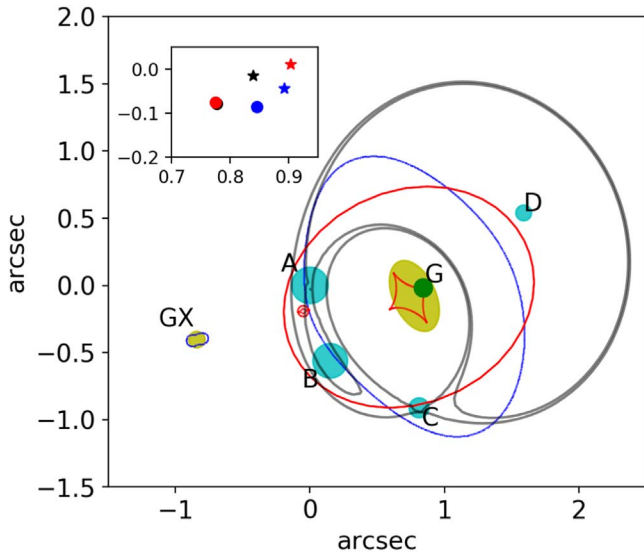
Figure 6. Lensing configuration for the SIE+ \gamma +GX model. The two lenses (G and GX) are marked with yellow ellipses whose sizes scale in proportion to the modeled velocity dispersions. The ellipsis for G shows the orientation and axis ratio predicted by the mass model. Critical lines are drawn in blue and caustics in red. The green circle marks the location of the source QSO in the source plane, and the cyan circles mark the locations of the observed images. The size of the circles is in proportion to the predicted flux ratios. Time delay surface isochrones at the location of the saddle point images A and C are drawn in gray. In the inset, the source QSO position (stars) and lens position (circles) are marked for the SIE+ \gamma +GX model (black), the SIE+ \gamma model (red), and the free SIE+ \gamma model (blue). The black circle coincides with the light profile centroid of the lensing galaxy.
