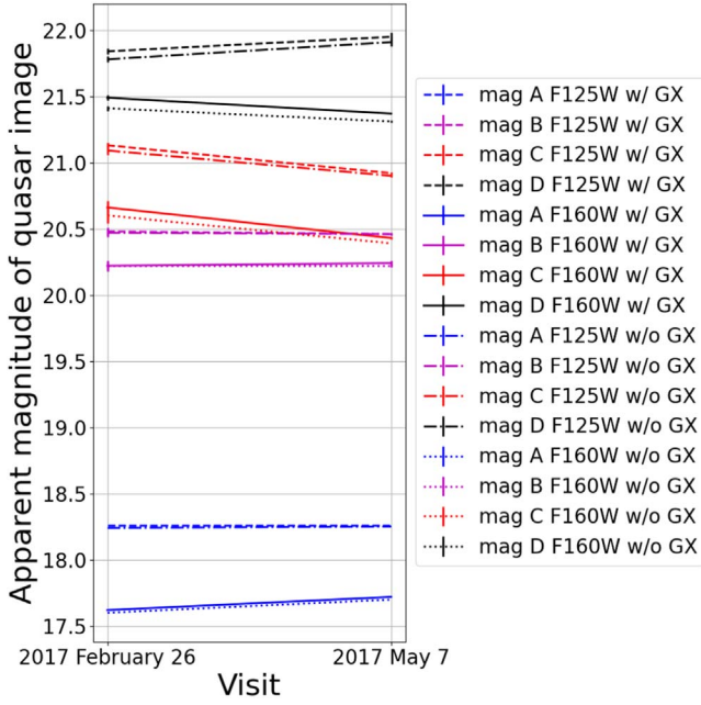
Figure 8. Variation of the QSO image magnitudes with observing epoch.
