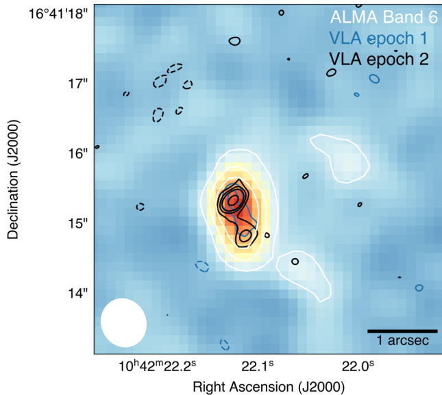
Figure 5. Radio (VLA) and submillimeter (ALMA) follow-up imaging. The blue image and black contours indicate the VLA emission at the first and second epochs, respectively. The white contours indicate the ALMA Band 6 emission. The contours are drawn at (-3, 3, 6, 9, 18, 36, 72, \text{ and } 144) times the off-source noise of each map, which is 6.7, 4.6, \text{ and } 62 \mu\text{Jy beam}^{-1} for the VLA epoch 1, VLA epoch 2, and ALMA observations, respectively. The restoring Gaussian beam of the ALMA observations is shown in white in the lower left corner and is 0''.64 \times 0''.57 with a PA of 23^\circ .
