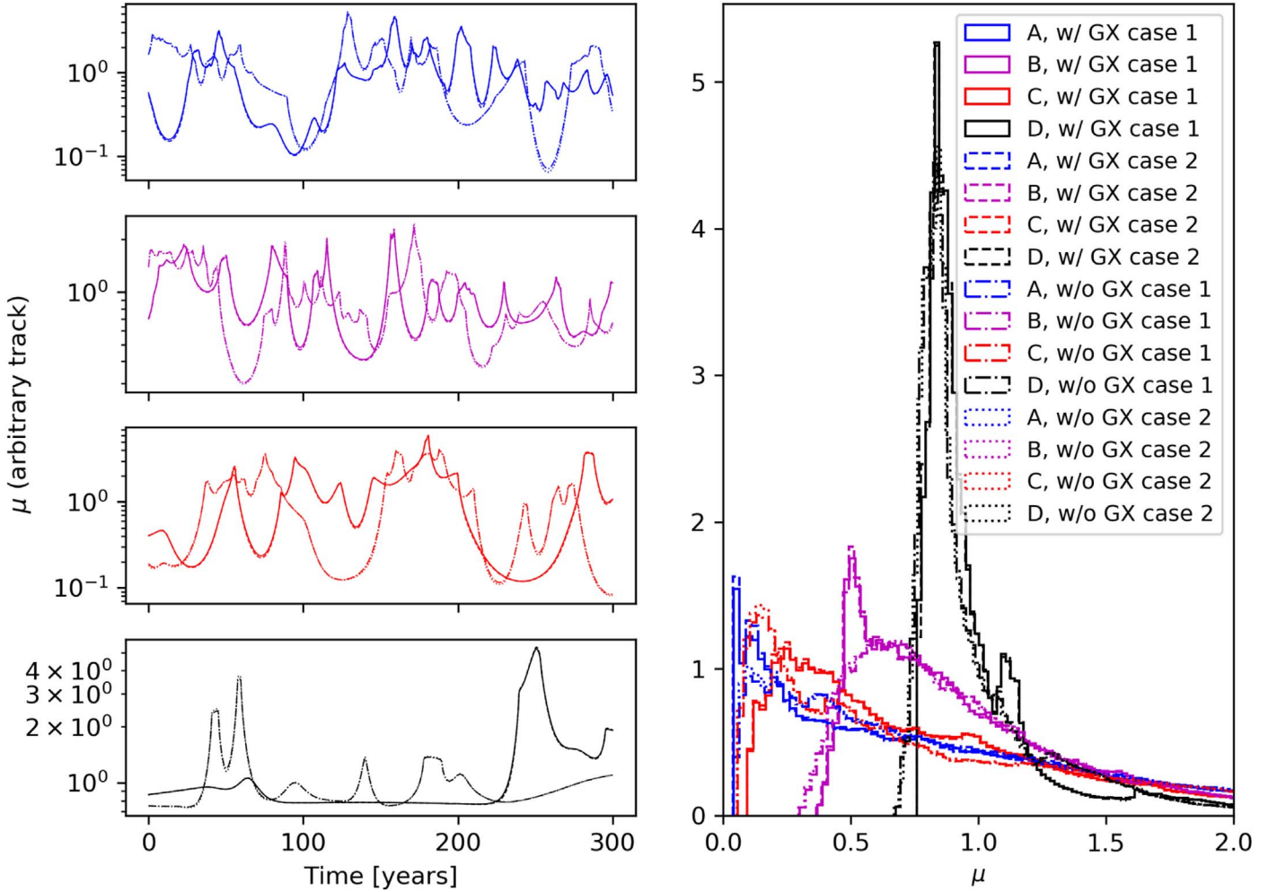
Figure 9. Simulated microlensing light curves in F160W. Left: magnification curves along an arbitrary track of the magnification maps of the four QSO images. The magnification of each image in the absence of microlensing has been normalized to unity by dividing over the magnifications predicted by two best-fit lensing models, SIE+ \gamma +GX and SIE+ \gamma with free lens position. The timescale is chosen to show the typical frequency of microlensing events for each image. Right: histograms of the microlensing magnification over the entire microlensing map. The histograms continue to decrease smoothly beyond the limit displayed. Case 1: \log M_{\text{BH}}[M_{\odot}] = 9.06 , L/L_{\text{Edd}} = 0.21 , \eta = 0.43 , R_0 = 2.76e+15 m; Case 2: \log M_{\text{BH}}[M_{\odot}] = 9.56 , L/L_{\text{Edd}} = 0.046 , \eta = 1.23 , R_0 = 2.52e+15 m. Both cases use 1.0R_0 , i = 60^\circ , and \text{PA} = 90^\circ . See Section B for further details.
