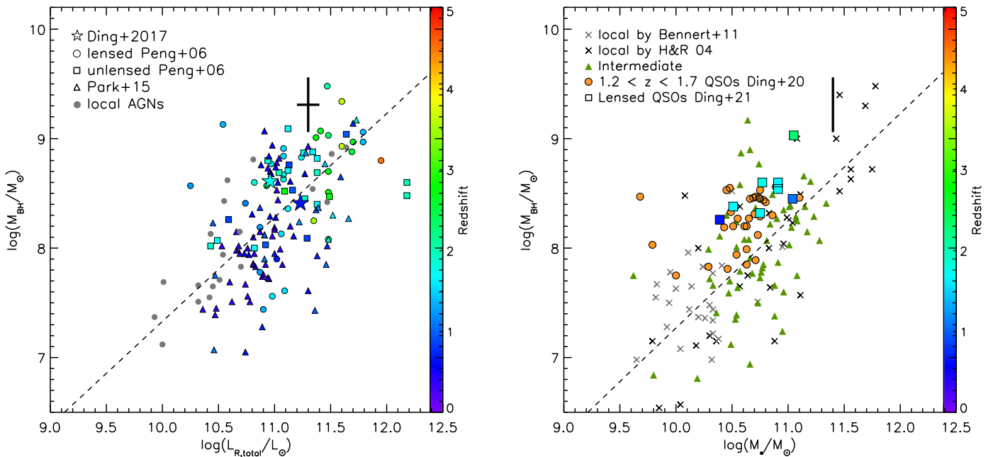
Figure 14. Left: Observed BH mass vs. total R -band host galaxy luminosity using data from lensed and unlensed AGNs across a broad redshift range (reproducing Figure 3 of Ding et al. 2017, which has not been corrected for passive evolution). Right: BH masses vs. stellar mass, as shown in Figure 3 of Ding et al. (2021). Sources are color-coded by redshift, and W2M J1042+1641 is represented by a thick black line spanning the possible values according to our calculations. The dashed black line is a fit to the local AGNs. In both figures, W2M J1042+1641 is above the local relation, and although it is the highest-redshift object with a stellar mass estimate, its offset from the local relation is consistent with the next-highest redshift source, HE 1104–1805 at z = 2.32 (green circle; Ding et al. 2021).
