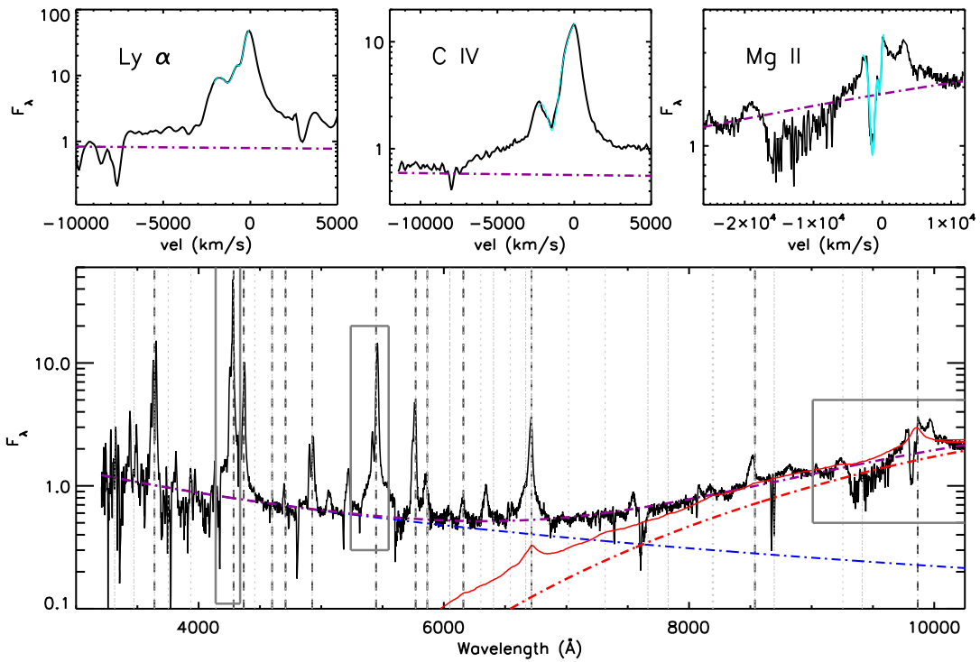
Figure 12. Deep LRIS spectrum of W2M J1042+1641 (bottom panel; black line), with typical (light gray) and prominent (dark gray) QSO emission lines marked with vertical dotted and dashed lines, respectively. A best-fit reddened power-law continuum plus an unreddened leakage component is shown with a purple dashed-dotted line, with the reddened ( E(B - V) = 0.89 ) and leaked components plotted in red and blue, respectively. The solid red line is the best-fit reddened template with E(B - V) = 0.73 . Top row: profiles of prominent emission lines Mg II, C IV, and Ly \alpha (left to right) plotted in velocity space. All three lines show a distinct absorption feature that is well fit by a single or double Gaussian profile, with an outflow speed of \sim 1000 – 1500 km s ^{-1} . We note that the absorption feature blueward of Mg II is due to telluric absorption. The line regions plotted in the squares at the top are also marked with gray boxes in the bottom panel.
