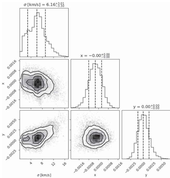
Figure 11. Velocity dispersion and position (in arcsec) of an SIS substructure added to the SIE+ \gamma +GX model around image A, in order to boost its flux by a factor of \sim 5 . The 16th and 84th velocity dispersion percentiles correspond to a mass (inside the substructure’s Einstein radius) of 4.1 \times 10^3 M_\odot and 4.3 \times 10^5 M_\odot , respectively.
