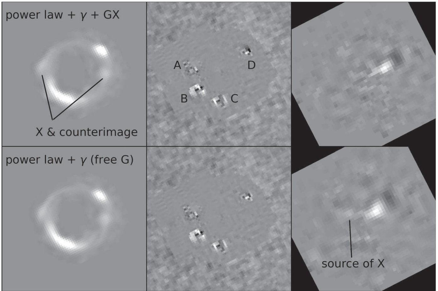
Figure 18. Pixel-based modeling of F125W visit 1 with g_lee (Suyu & Halkola 2010; Suyu et al. 2012). A power-law + \gamma +GX mass model was used for the top panels, and a power-law + \gamma model with free lens position was used for the bottom panels. From left to right: the best-fit model of the extended arcs, the residuals after subtracting the best-fit model (the gray scale is linear, from -10\sigma to 10\sigma ), and the source reconstruction on a 50 \times 50 pixel grid. The pixel scales in the source plane averaged between the two axes are 0''.030 (top) and 0''.024 (bottom). North is up, and east is to the left. Note in the arc the luminous blob, X, south of image D, and its fainter counterimage situated on the diametrically opposed part of the arc. The QSO host appears elongated with a possible tidal tail extending toward the less luminous substructure on the left, responsible for the luminous blob seen in the arc.
