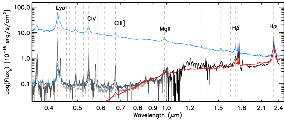
Figure 1. Optical through near-infrared spectrum of W2M J1042+1641, plotted on logarithmic wavelength and flux axes. The black line at \lambda > 1 \mu\text{m} is the near-infrared spectrum, showing broad Balmer line emission shifted to z = 2.517 . The dark-gray line is the LBT optical spectrum, and the light-gray line is the LRIS spectrum (Section 2.4), showing the consistency between the two spectra taken 5 yr apart (observed frame). Vertical dashed lines mark the locations of strong emission lines seen in the spectrum. The red line is the best-fit QSO template (shown in blue) reddened by E(B - V) = 0.68 to the LBT spectrum combined with the near-infrared spectrum. In both cases, the rest-frame UV part of the spectrum deviates from the reddened template, implying that the obscuring dust is shielding most of the central region but allows \sim 0.8\% of the intrinsic emission to enter our line of sight (blue dashed line).
