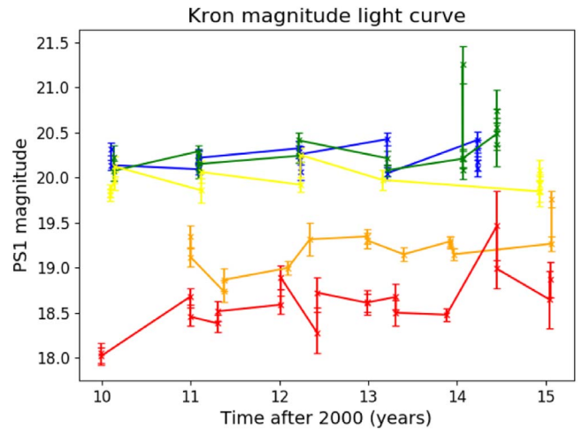
Figure 10. Variability of W2M J1042+1641 in individual Pan-STARRS1 exposures. Blue, green, yellow, orange, and red colors represent, in order, grizy . Mismatches in photometry between points very close in time suggest that the photometric errors are underestimated, weakening evidence for variability. Note that the SDSS magnitudes from Table 1, taken earlier in time, are in relatively good agreement.
