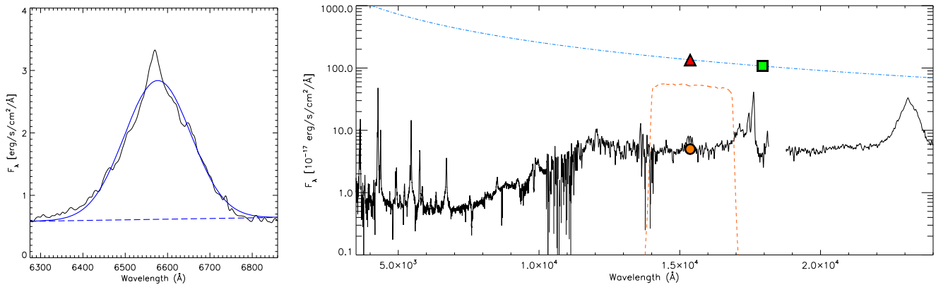
Figure 13. Left: we show the H\alpha line, seen in the near-infrared spectrum (black line), fit with a single Gaussian plus a linear continuum fit (solid blue line) to determine the FWHM needed to compute the BH mass in Equation (4). The linear continuum is shown with a dashed blue line. Right: we scale our spectrum to the total F160W flux from the QSO (orange circle). We plot the dereddened continuum from Equation (3) (cyan dotted–dashed line) and shift from the observed flux through the F160W band to match the dereddened continuum (red triangle) to the flux at 5100 Å flux (green square). We use this value to find L_{5100} and compute the BH mass in Equation (4).
