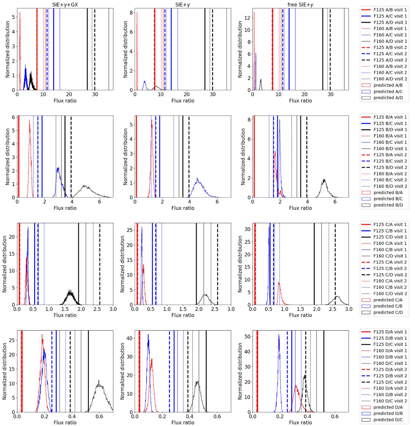
Figure 7. Comparison of observed and predicted flux ratios. The lens mass models, from left to right, are SIE+ \gamma +GX, SIE+ \gamma , and free SIE+ \gamma . The histograms consist of 10,000 points from the MCMC chains computed with glafic , and the vertical lines correspond to the photometry measured by hostlens . Visits: (1) UT 2017 February 26; (2): UT 2017 May 7. The fluxes of image D in visit 2 may be unreliable owing to a diffraction spike from image A falling on top of it.
