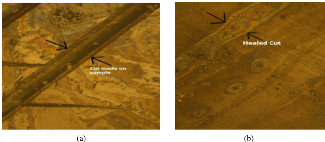
Fig. 4. Epoxy composite with 60:40 DETA:PDMS ratio and 0.1% GO: (a) before self-healing and (b) after self-healing (at 110 °C)
