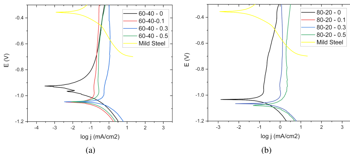
Fig. 5. Tafel Polarization Curves of working electrode potential vs current density depicting (a) self-healing composites with DETA:PDMS ratio of 60:40 with varying amounts of GO coated on mild steel and (b) self-healing composites with DETA:PDMS ratio of 80:20 with varying amounts of GO coated on mild steel. The polarization curve of uncoated mild steel sample is given with both for reference
