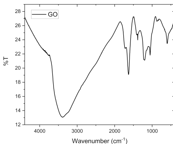
Fig. 1. FTIR Spectroscopy analysis of GO sample
