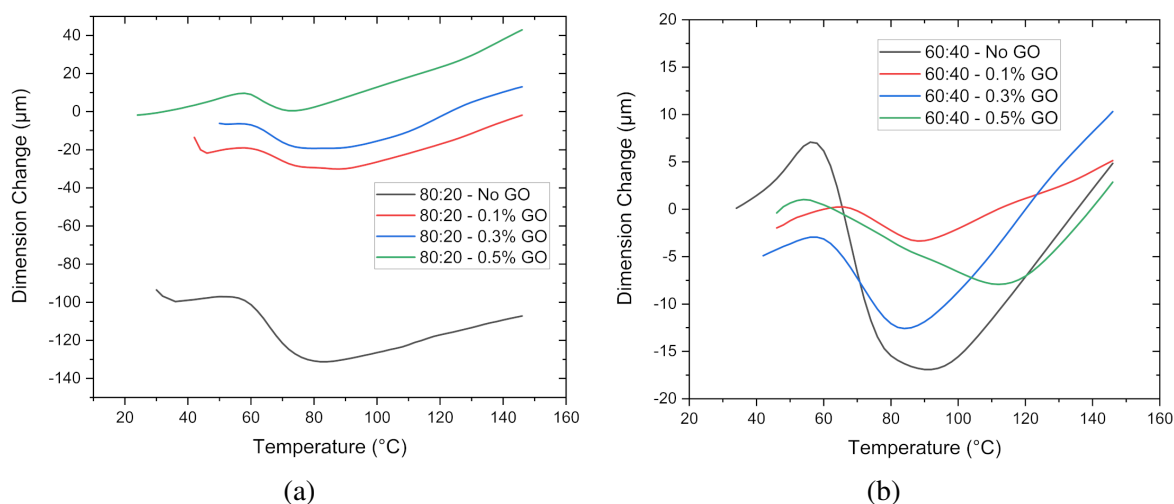
Fig. 3. Thermo-mechanical analysis graphs of (a) epoxy composite with 80:20 DETA:PDMS ratio and (b) epoxy composite with 60:40 DETA:PDMS ratio
