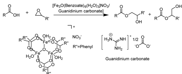
Scheme 1 Reported LA/LB cooperative catalyst systems for the nucleophilic ring opening of epoxides by carboxylic acids; (a) iron or chromium salts in conjunction with amines, 65 (b) FeCl 3 /pyridine 66 and (c) this work: the ([Fe 3 O(benzoate) 6 (H 2 O) 3 ]NO 3 )/guanidinium carbonate catalyst system.
